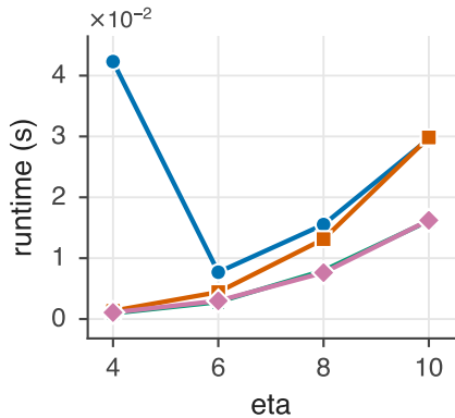
local two-svd timing
