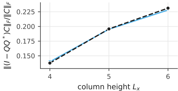
...not by the probe count \ell (at \eta_q = 4 )
