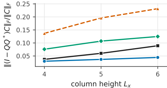
Accuracy is set by the vertical bond \eta_q
