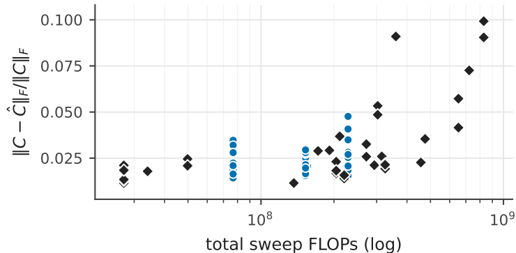
Pareto: error vs propagated cost (0/36 near-full-rank)
