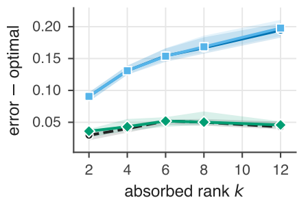
Excess over Eckart-Young
