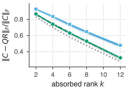
Column error (+ EY floor)
