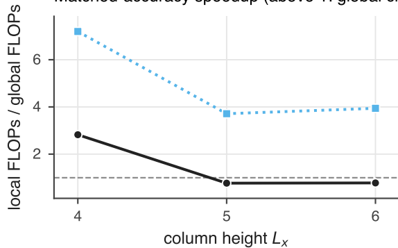
Matched-accuracy speedup (above 1: global cheaper)
