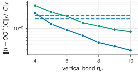
Global sketch: projection error vs vertical bond \eta_q
