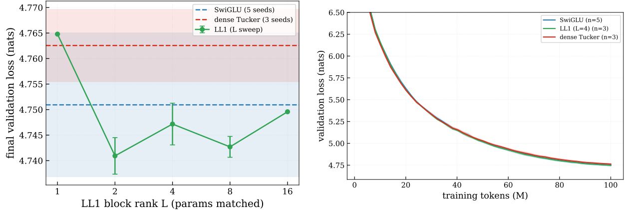
Figure 4: Matched-budget language modeling (52.5M parameters, 100M FineWeb-Edu tokens). Left: final validation loss across the LL1 block-rank sweep (error bars = std over 3 seeds at L \in \{2, 4, 8\} ; L \in \{1, 16\} single-seed), with SwiGLU ( n=5 , blue) and dense Tucker ( n=3 , red) mean \pm std bands. Every L \geq 2 sits below the SwiGLU mean but within its band: a statistical tie. Right: validation-loss curves (mean \pm std) — the three families are indistinguishable through training.
