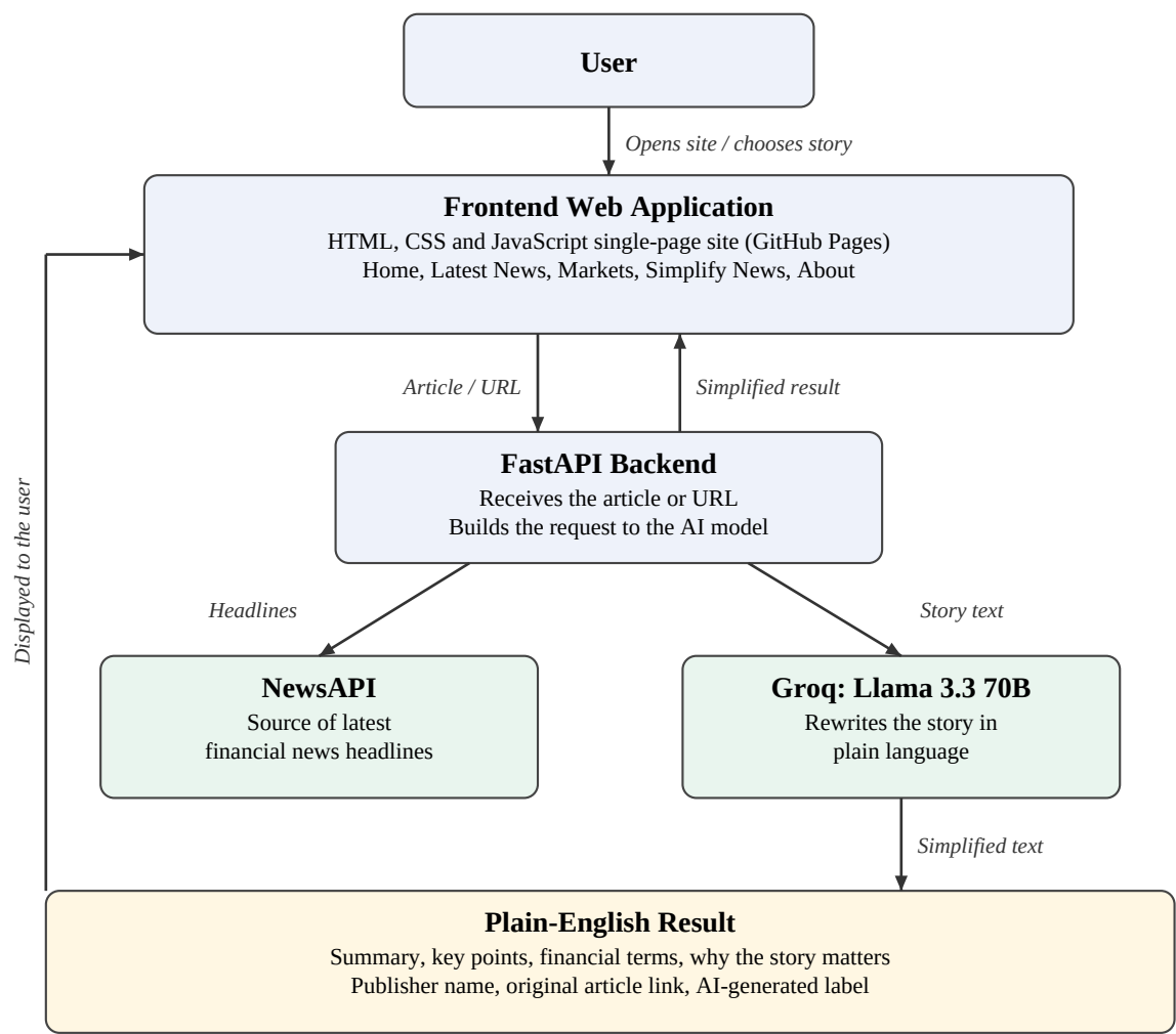
Figure 1: Technical Architecture of FinNews AI
