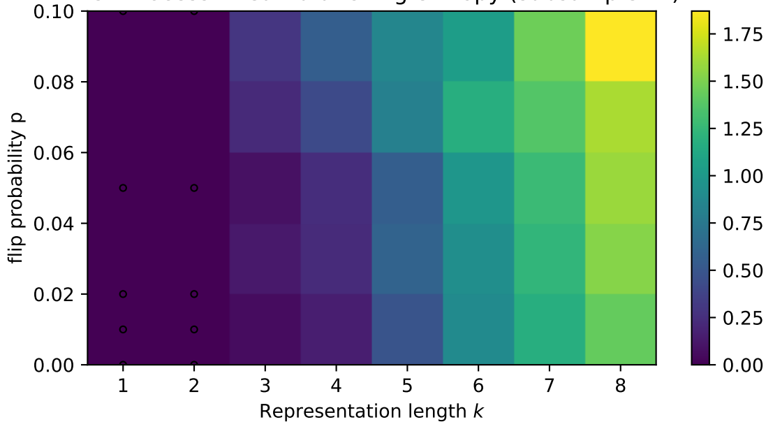
Even Process: mean branching entropy (subsample=4)
