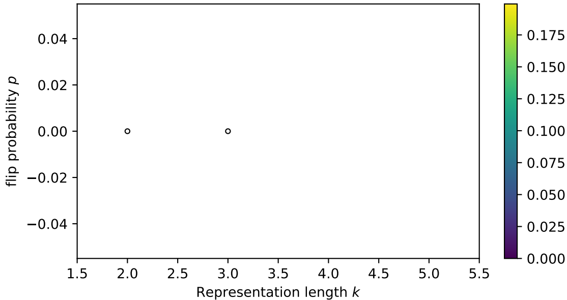
mean 1 – unifilarity (subsample=1)
