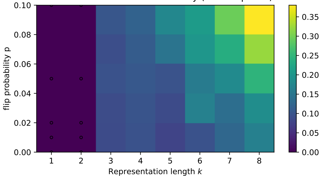
Even Process: mean 1 – unifilarity (subsample=1)
