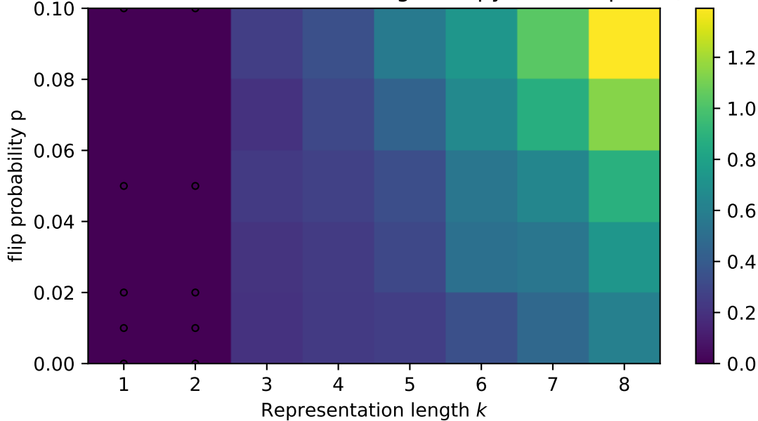
Even Process: mean branching entropy (subsample=1)
