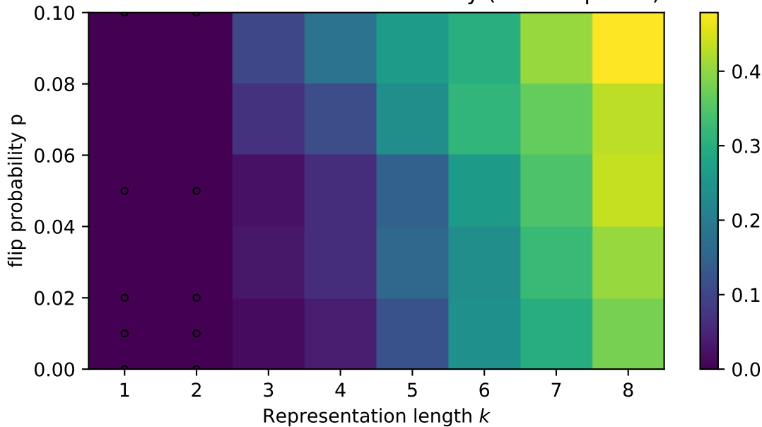
Even Process: mean 1 – unifilarity (subsample=4)
