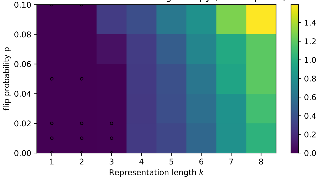
Even Process: mean branching entropy (subsample=2)
