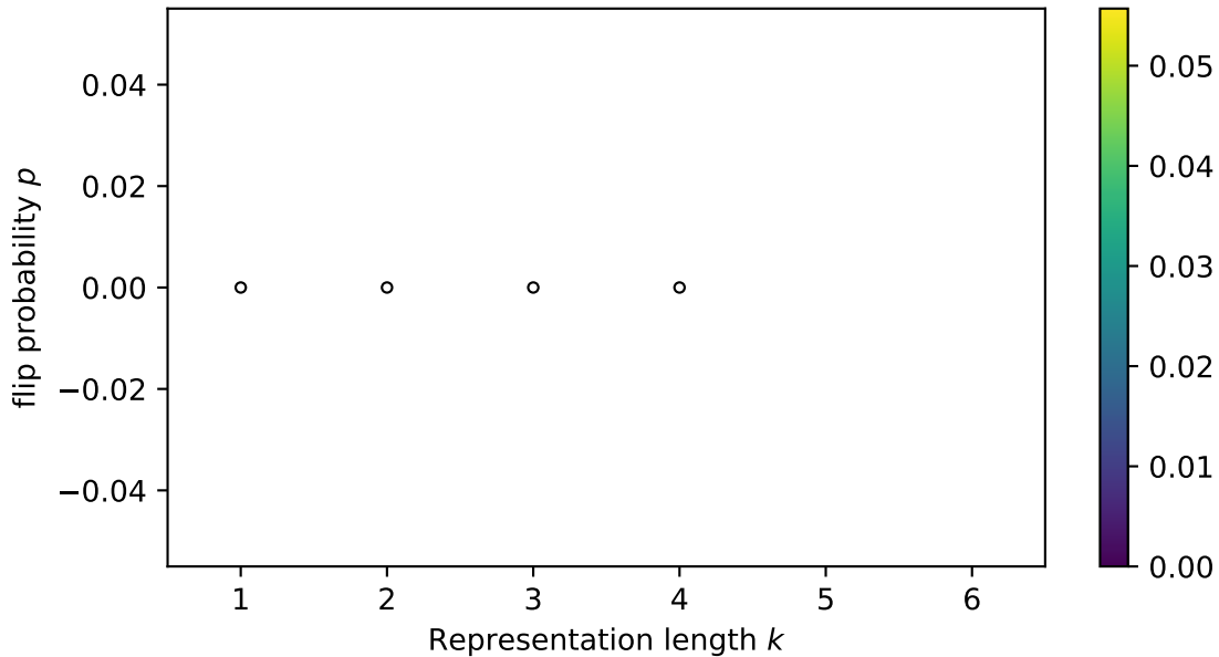
mean 1 – unifilarity (subsample=1)
