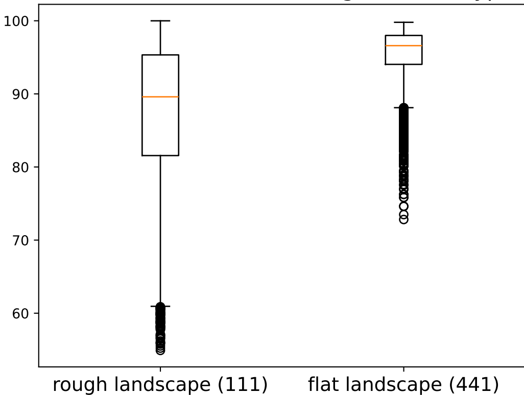
QNN Loss Landscape values (Schmidt Rank, size training set, data type)
