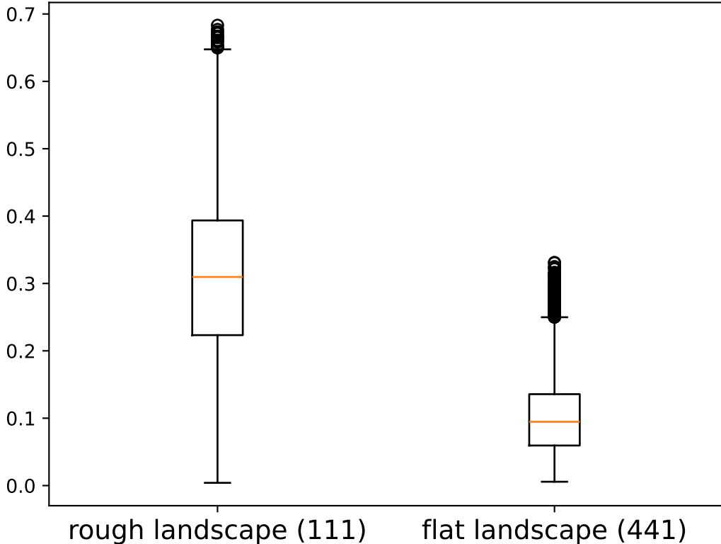
QNN Loss Gradients (norm) (Schmidt Rank, size training set, data type)
