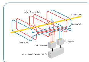
APEX 500 Metal Detector Multi/Coil Architecture
