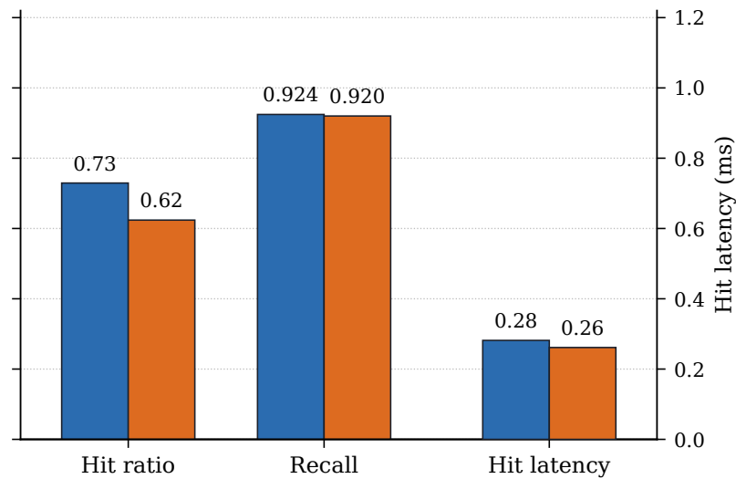
simZipf+ ( \lambda = 0.01 )
