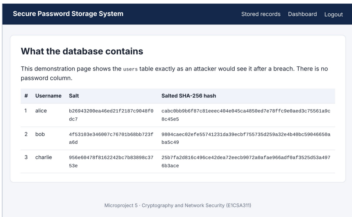
Figure 4.14: Web interface: contents of the users table (alice and bob have the same password)
