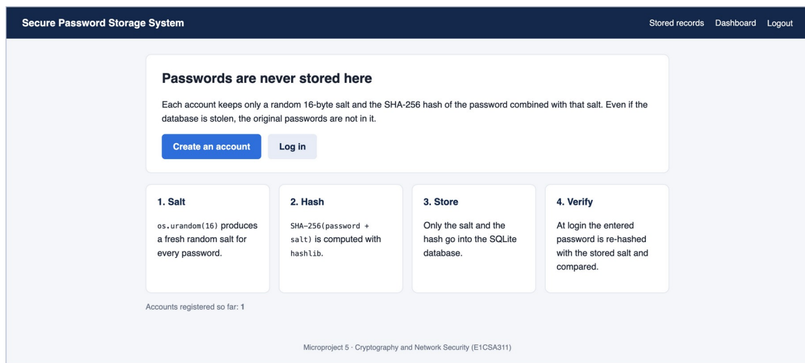
Figure 4.10: Web interface: home page, served at http://127.0.0.1:5000
