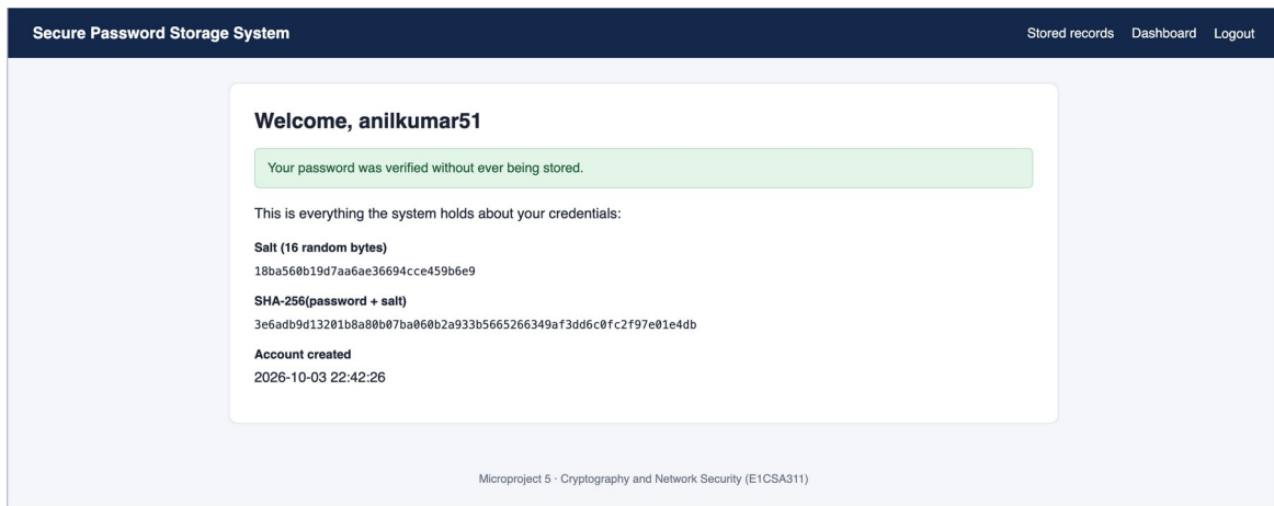
Figure 4.13: Web interface: dashboard after a successful login
