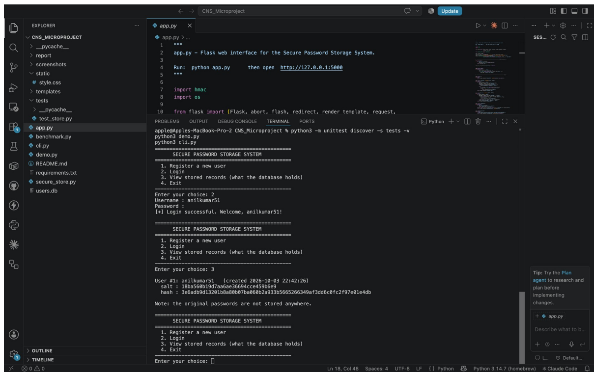
Figure 4.15: The project in Visual Studio Code on macOS, with cli.py running in the integrated terminal (login and stored records)
