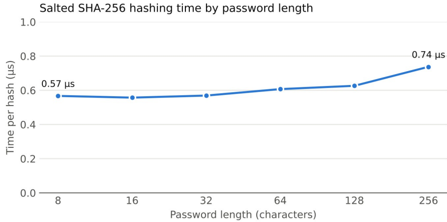
Figure 4.1: Salted SHA-256 hashing time for different password lengths
