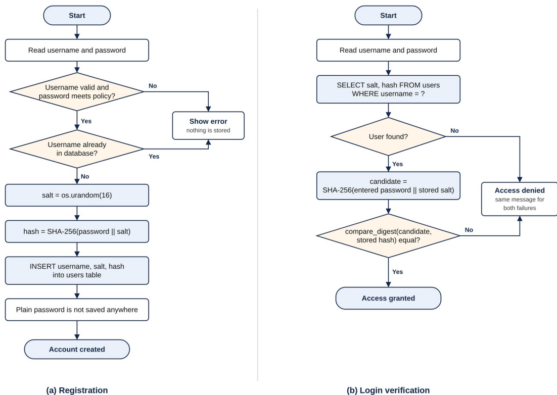
Figure 2.2: Flowcharts of (a) registration and (b) login verification
