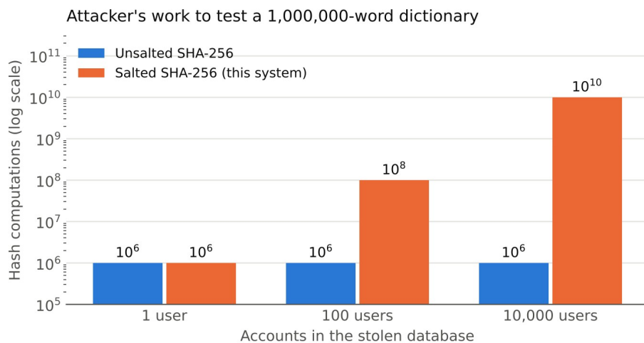
Figure 4.2: Attacker's work with and without salts (logarithmic scale)
