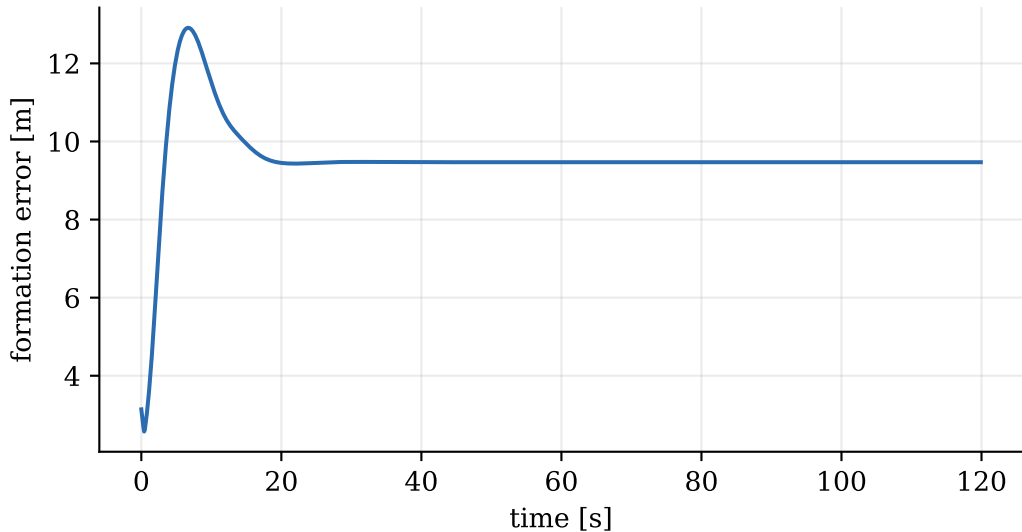
Fixed-wing coordinated-turn formation error
