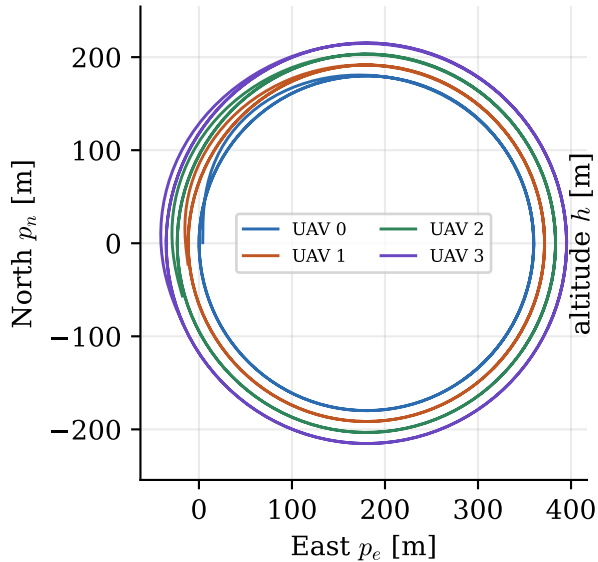
Fixed-wing formation (top view)
