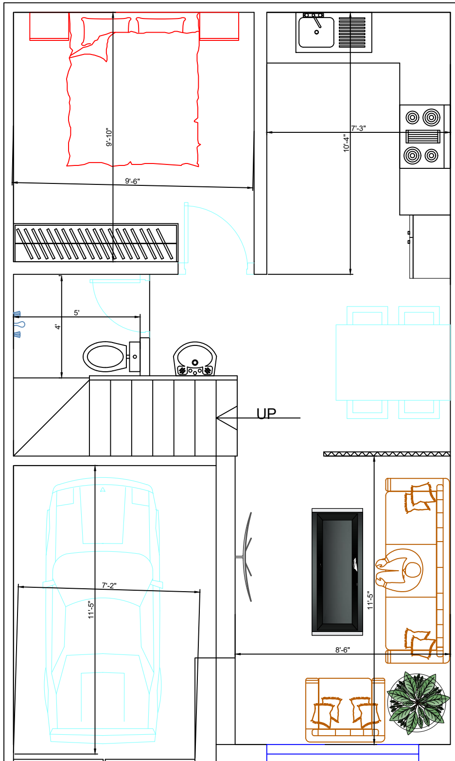
GROUND FLOOR ALT NO :- 01
