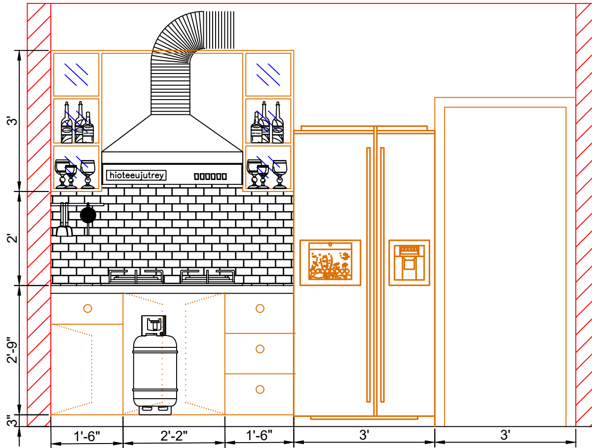
Elevation A Internal
