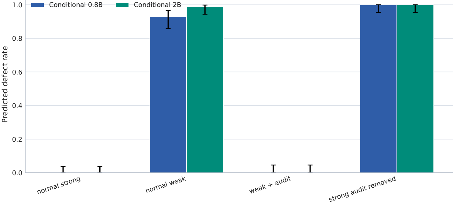
Counterfactual audit direction
