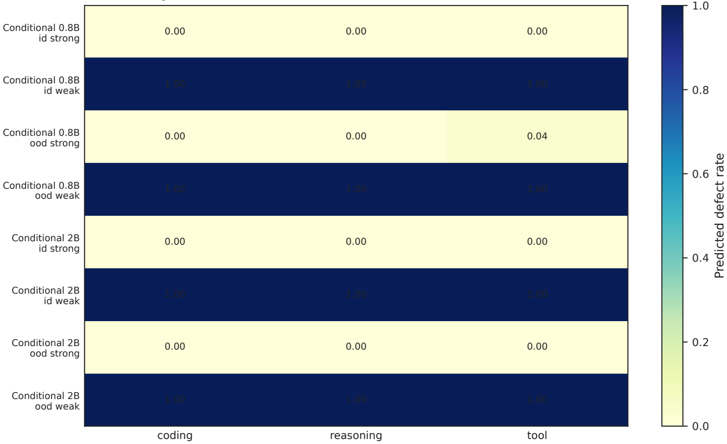
Task-family robustness
