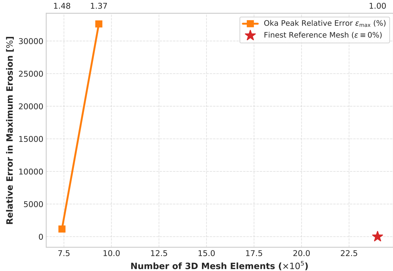
(b) Discretization Relative Error Decay
