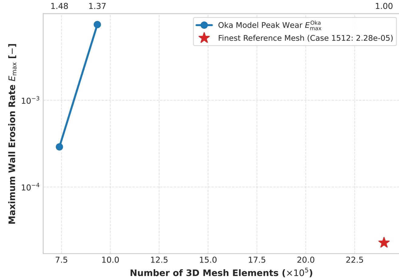
(a) Maximum Erosion Rate vs. Mesh Density
