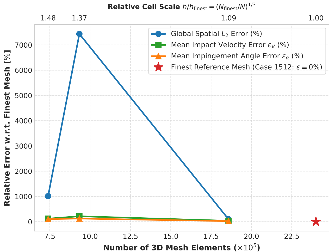
(b) Discretization Error Decay vs. Mesh Density
