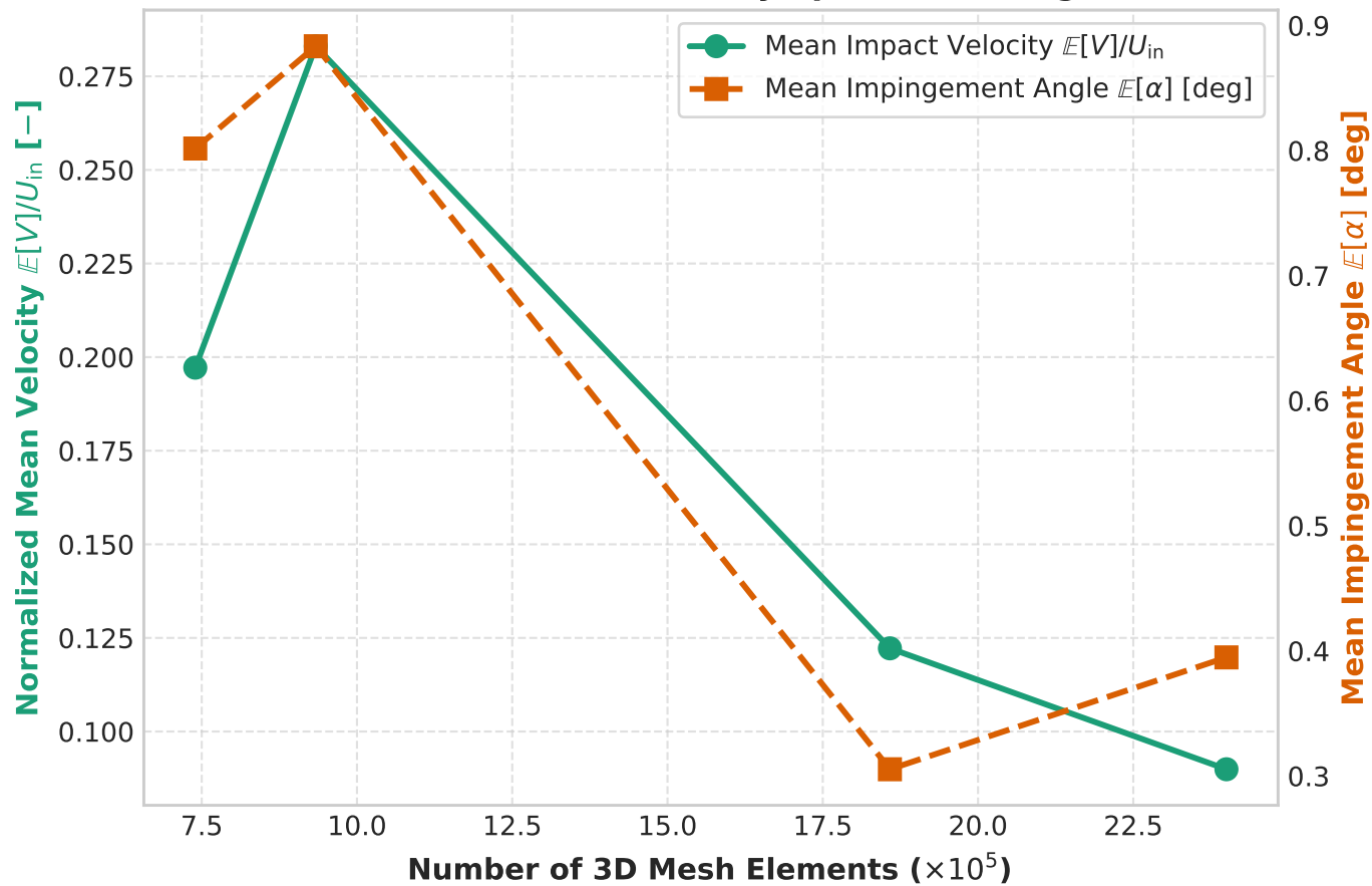
(a) Kinematic Parameter Asymptotic Convergence
