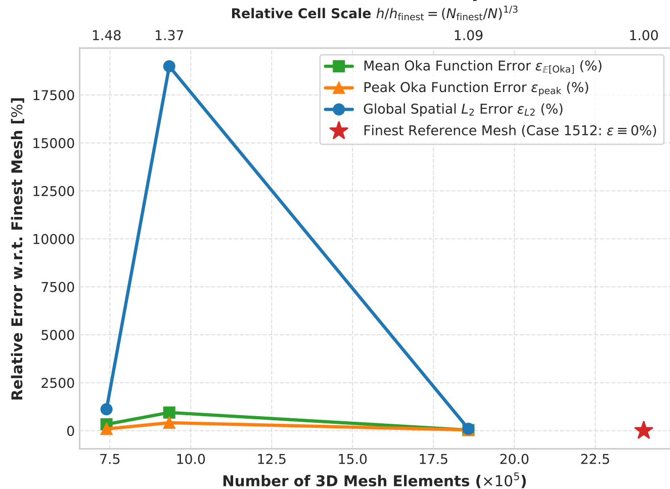
(b) Oka Erosion Discretization Error Decay vs. Element Count
