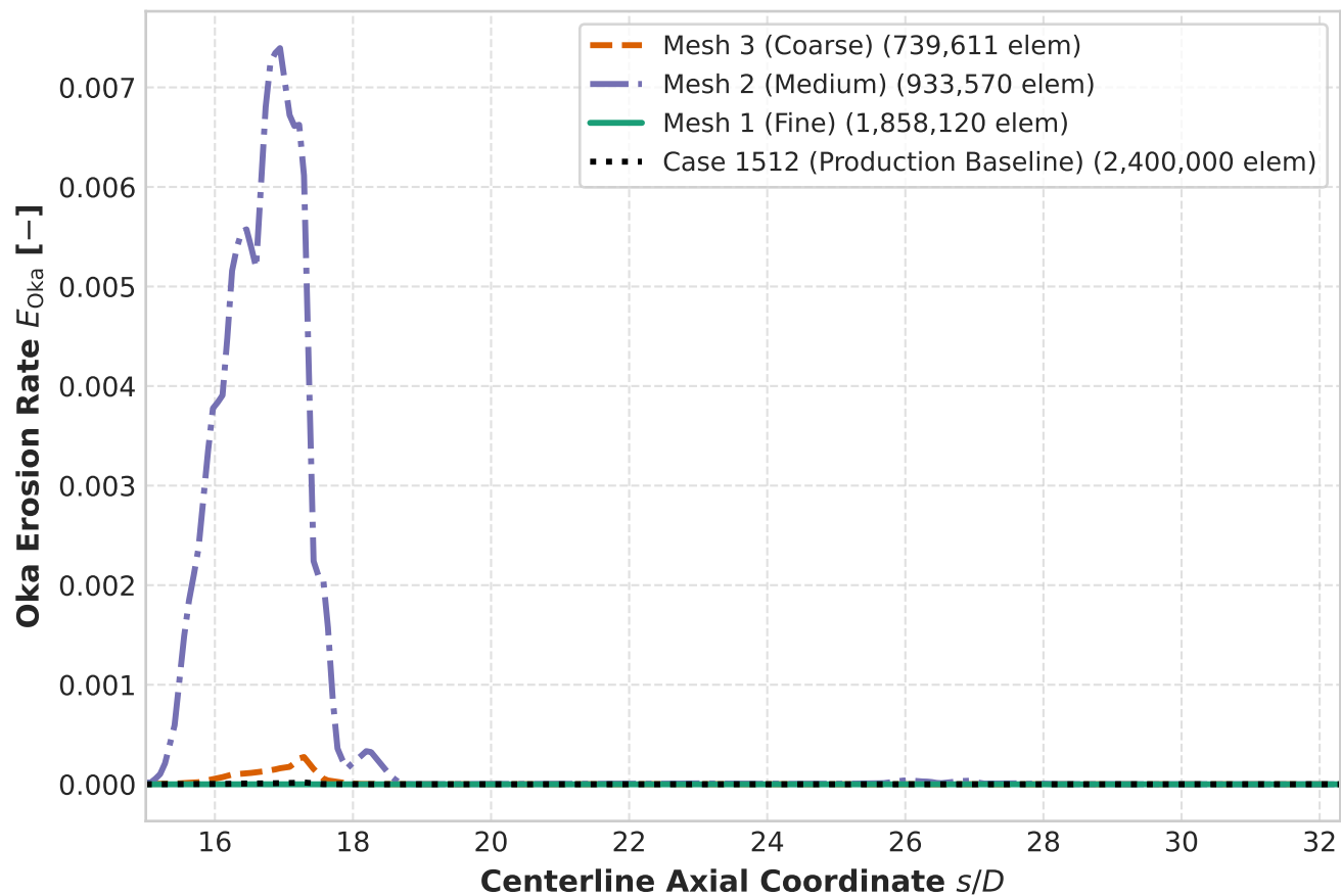
(a) Extrados Centerline Oka Erosion Profile ( \theta = 0^\circ )
