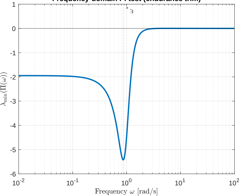
Frequency-domain PI test (endurance trim)
