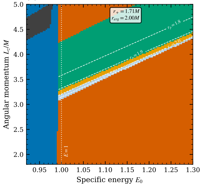
(a) a/M=0.7
