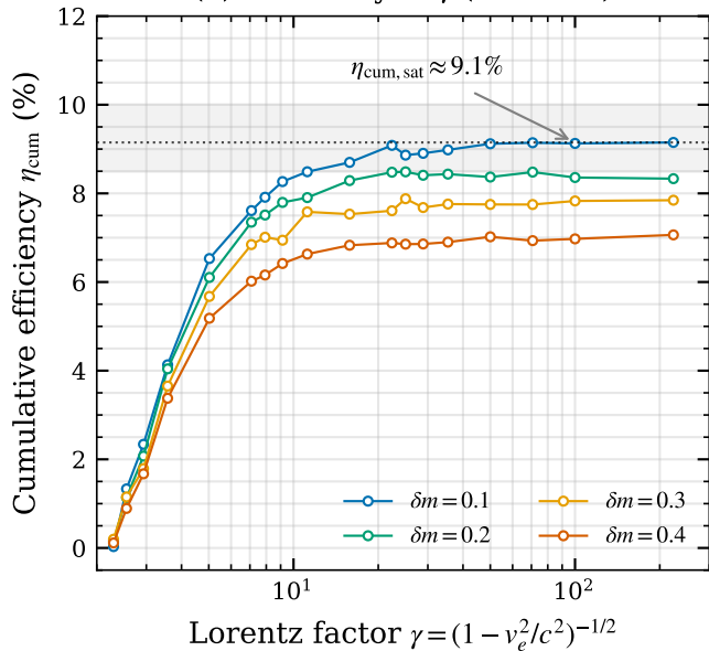
(a) Efficiency vs \gamma ( a/M=0.95 )
