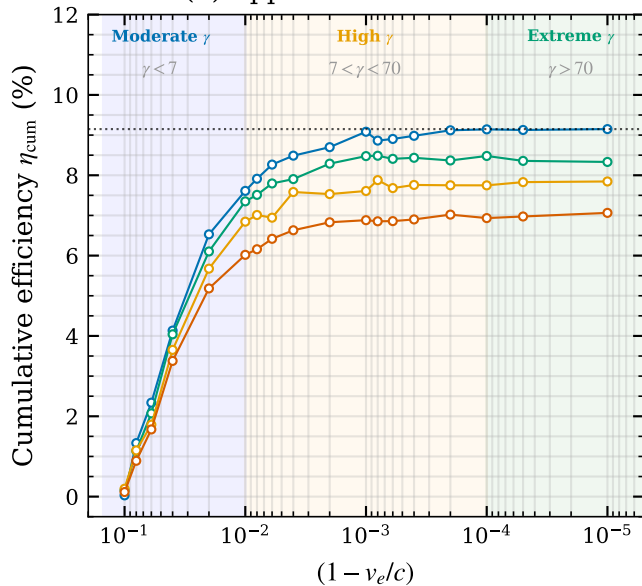
(b) Approach to Saturation
