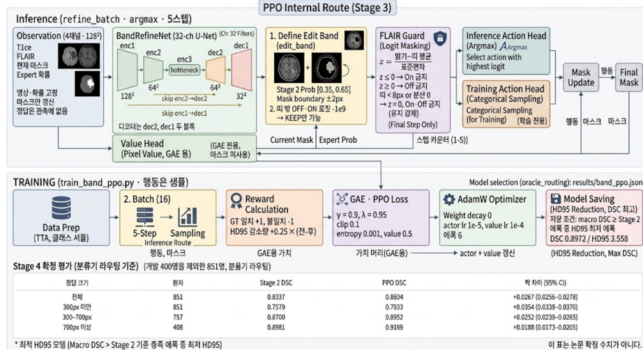
Fig. 2. Internal route of the boundary-band PPO. The upper path is five-step argmax inference. The lower path is training: reward, GAE-PPO loss, and the AdamW update of the action and value heads. The table at the bottom is the locked evaluation on 851 patients with classifier routing.
