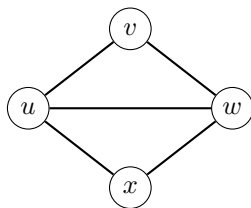
(a) G = (V, E) with V = \{u, v, w, x, \dots\} and E = \{(u, v), (v, w), \dots\} .
