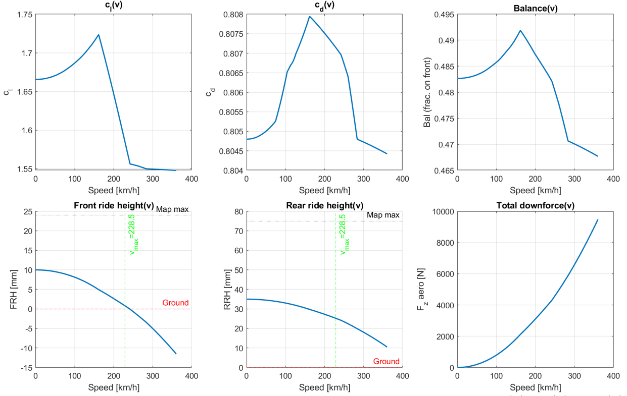
Figure 5.3: Aero quantities of the winning setup as a function of speed: c_l(v) , c_d(v) , Bal(v) , FRH(v) , RRH(v) and total downforce. The green dashed line marks the maximum speed reached on the lap, the red dashed line marks the ground.
