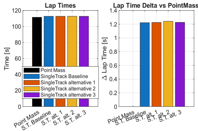
Figure 4.7: Lap times of the bicycle model with the four different braking systems compared to the single point mass simulation
