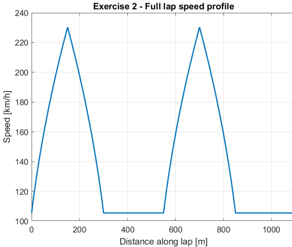
Figure 1.2: Full speed profile along the oval trajectory.
