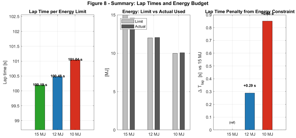
Figure 7.1: Summary of the three scenarios: lap time (left), energy limit vs. actual consumption (centre), and lap-time penalty relative to the 15 MJ reference (right).
