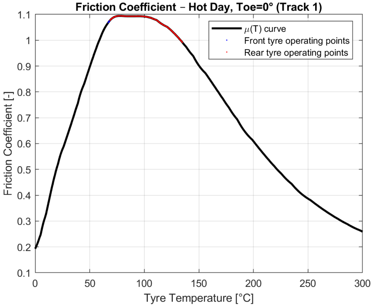
Figure 2.4: Friction coefficient \mu(T) curve (black) with operating points of front (blue) and rear (red) tyres for the Hot Day reference case.
