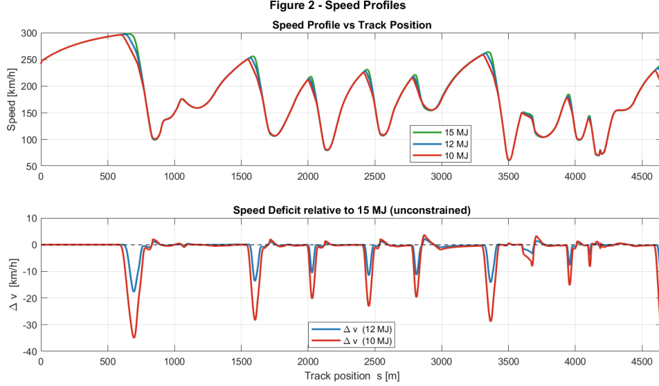
Figure 7.3: Speed profiles (top) and speed deficit relative to the 15 MJ reference (bottom) vs. track position. Negative values indicate where the energy-limited car is slower.
