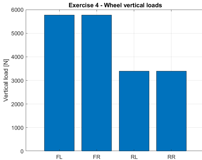
Figure 1.6: Vertical load on each wheel under braking.
