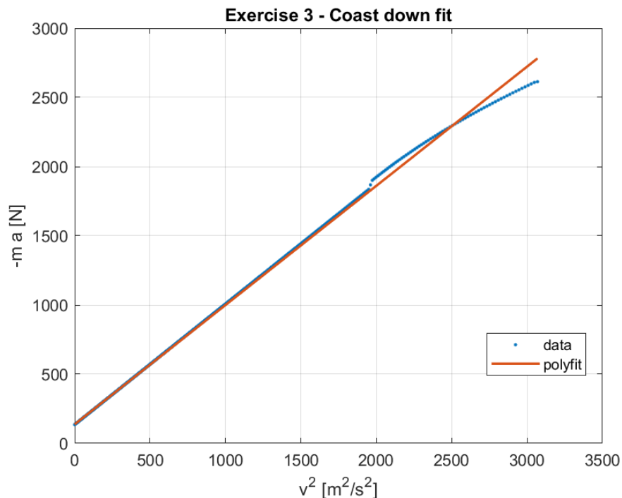
Figure 1.4: Linear fit of -m a_x vs. v^2 via polyfit. The slope gives A and the intercept B .
