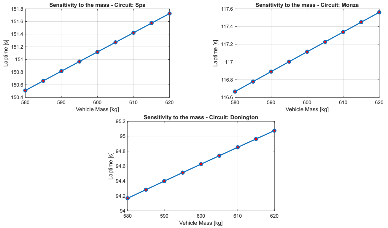
Figure 3.1: Sensitivity to the vehicle total mass (car+fuel) with cd = 1 and cl = 0.6
