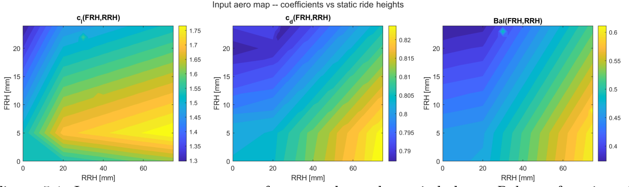
Figure 5.1: Input aero map: contours of c_l , c_d and aerodynamic balance Bal as a function of front and rear static ride height.
