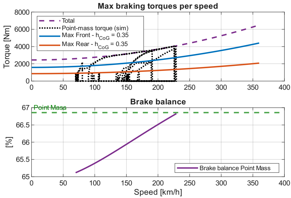
Figure 4.3: Max longitudinal torques compared with simulation and Ideal brake balance depending on speed
