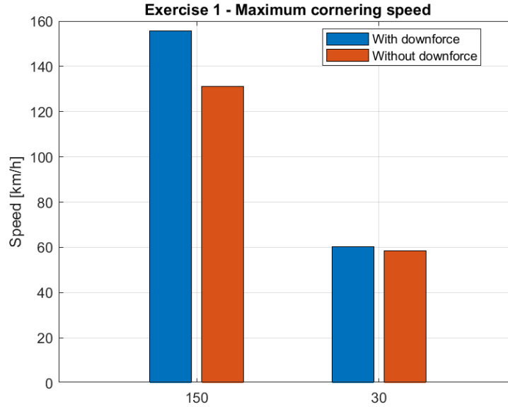
Figure 1.1: Maximum cornering speed with and without downforce for R = 150 m and R = 30 m.
