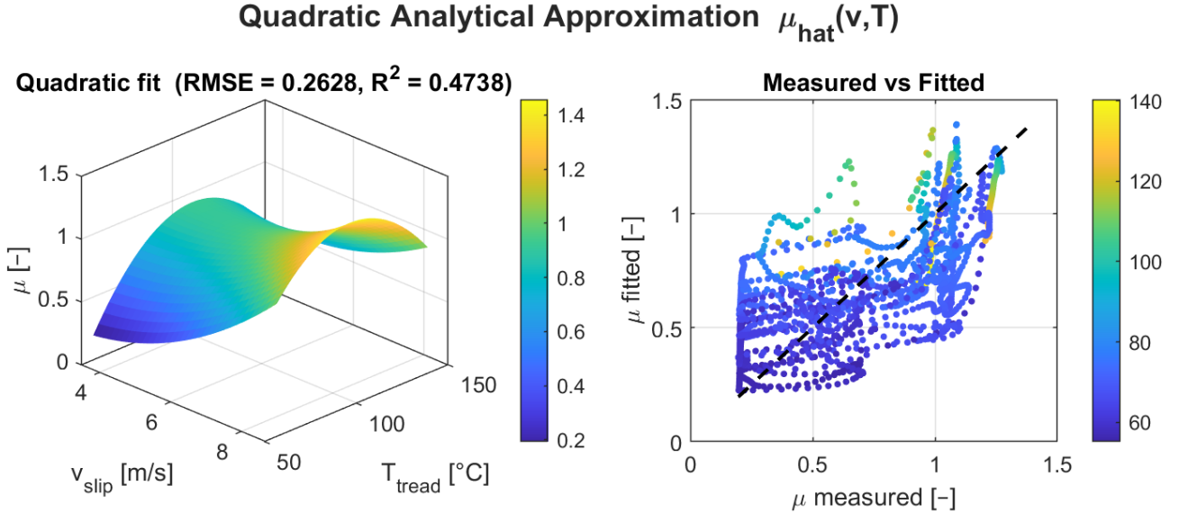
Figure 2.14: Quadratic analytical fit \hat{\mu}(v, T) (Eq. 2.9). Left: fitted surface. Right: measured vs. fitted values (identity line in black dashed).
