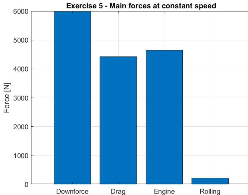
Figure 1.8: Force breakdown at 250 km/h: engine traction, drag, rolling resistance, and total downforce.
