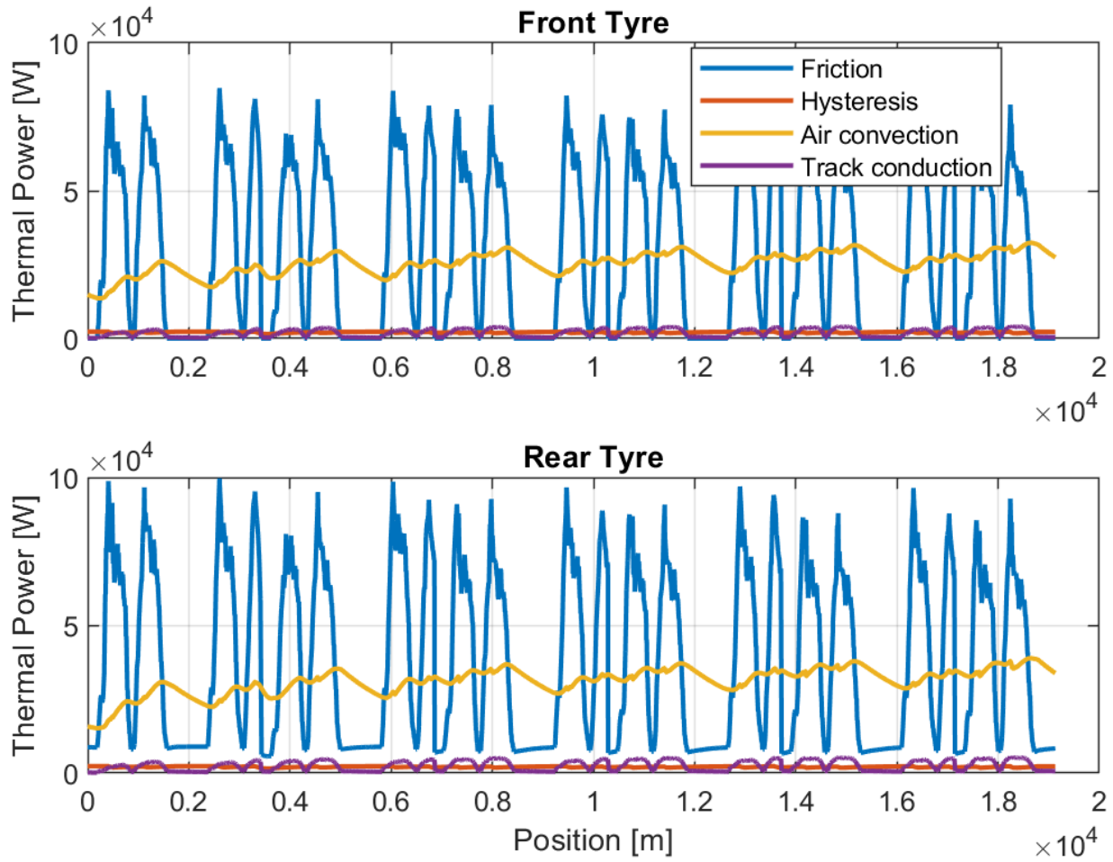
Figure 2.7: Thermal power breakdown for front (top) and rear (bottom) tyres at the reference set-up ( WD = 50\% , AB = 50\% , Hot Day).
