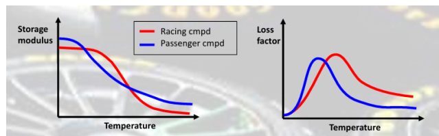
Figure 8.6: Storage modulus and loss energy comparison between racing and passenger compounds
