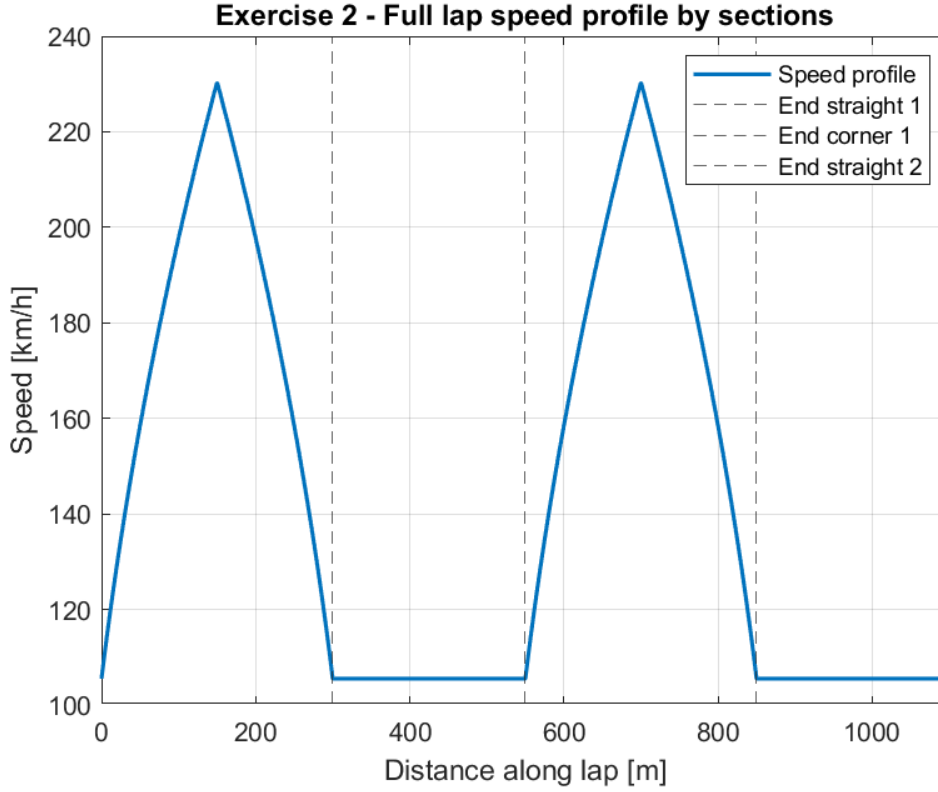
Figure 1.3: Speed profile with section annotations (acceleration, braking, corner).
