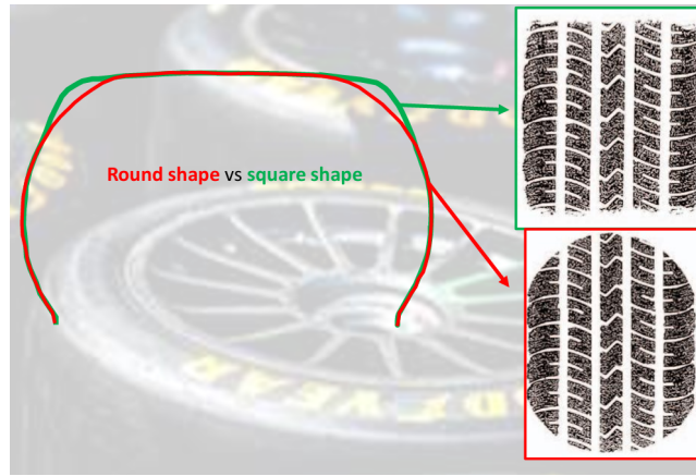
Figure 8.5: Tire footprints for round and square shapes
