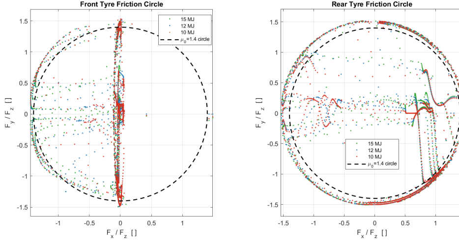
Figure 7.7: Friction-circle scatter for front (left) and rear (right) axles. The dashed circle is \mu_0 = 1.4 ; points outside it are admissible because the load-dependent friction limit is larger at this car's operating loads.
