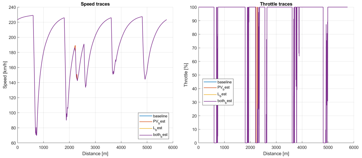
Figure 5.5: Speed (left) and throttle (right) traces along the lap for the four representative cases. The cuts in throttle correspond to the lift windows in Prima Variante and Lesmo 1.
