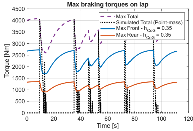
Figure 4.1: Braking torques computed with the bicycle model compared with the poin-mass model
