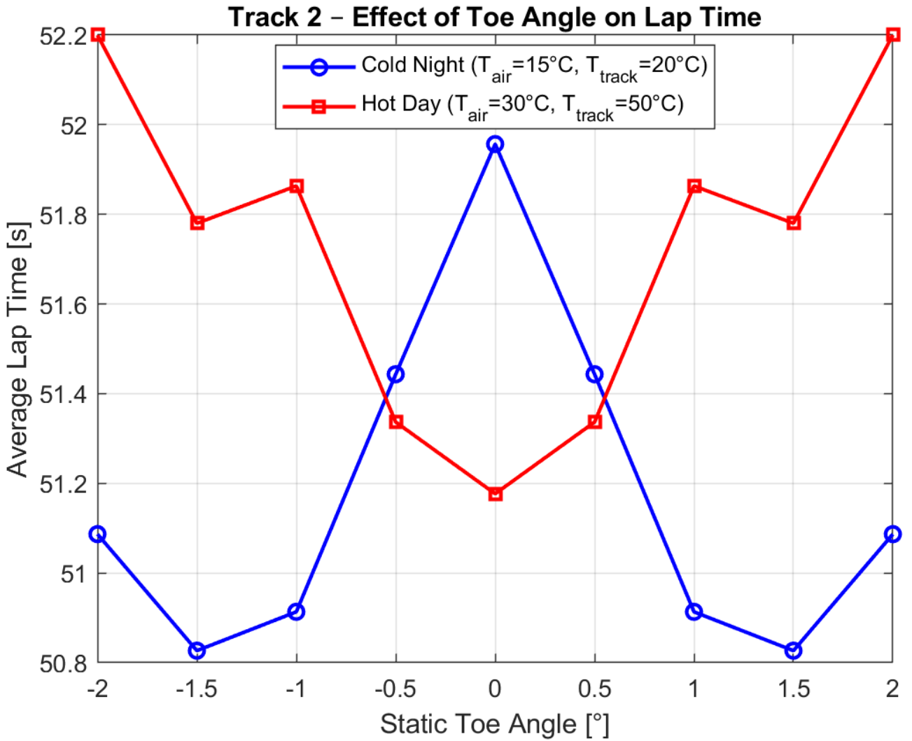
Figure 2.2: Average lap time vs. static toe angle on Track 2 (same format as Figure 2.1).
