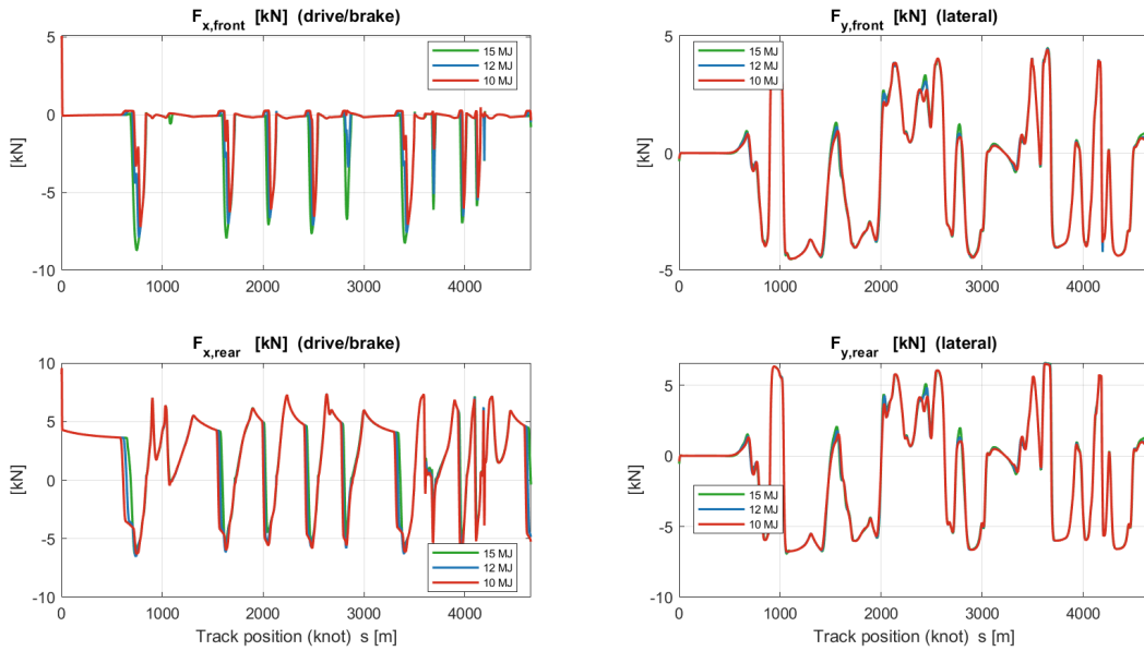
Figure 7.8: Tyre forces at knot points: longitudinal and lateral components for front and rear axles, with the three energy cases superimposed.
