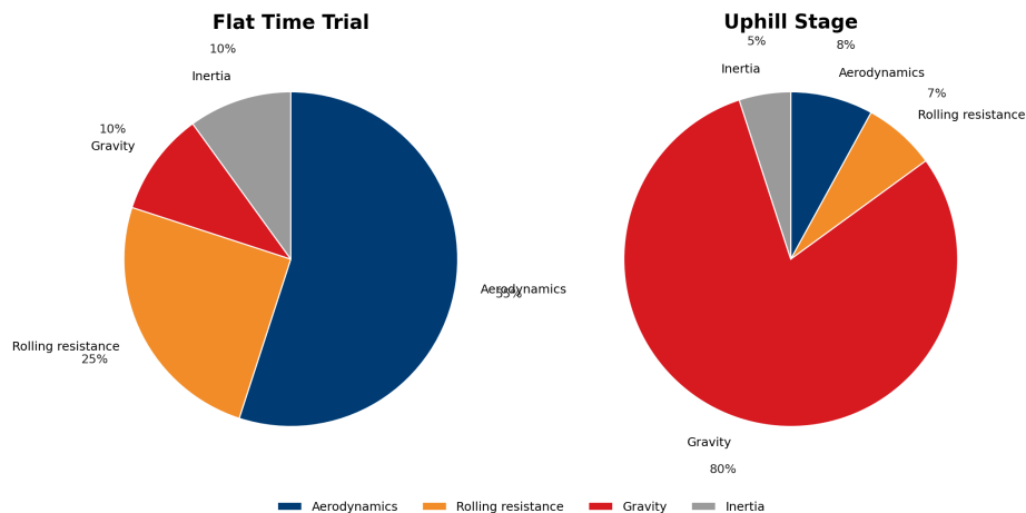
Figure 8.14: Energy balance breakdown for a flat time trial (left) and an uphill stage (right): aerodynamics dominates on the flat while gravity dominates on climbs. Pirelli Cycling R&D.
