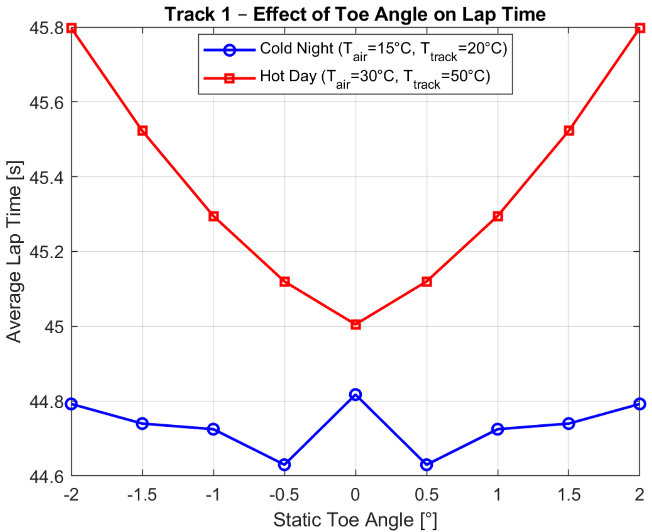
Figure 2.1: Average lap time as a function of static toe angle on Track 1 for the Cold Night (blue) and Hot Day (red) conditions.
