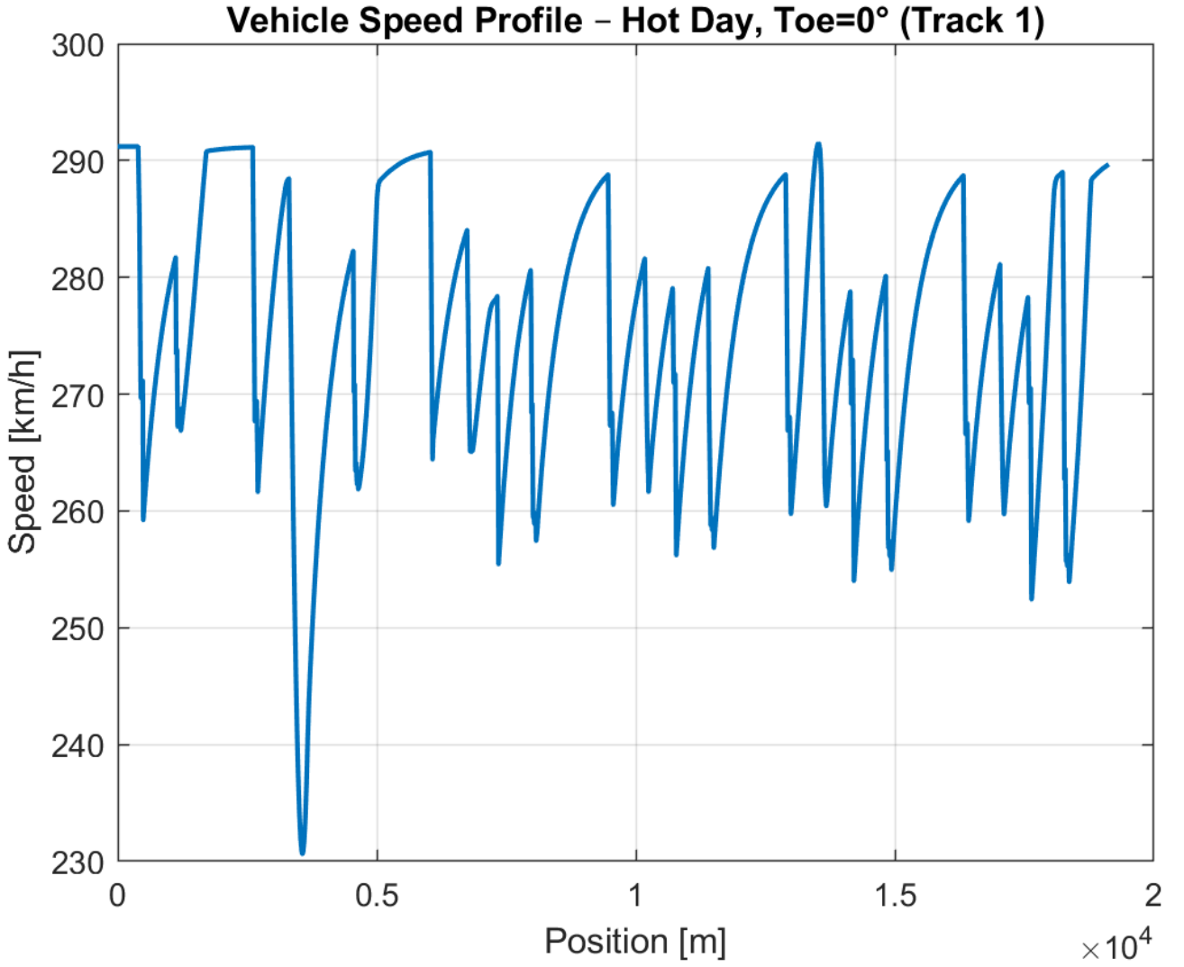
Figure 2.8: Vehicle speed profile as a function of track position for the Hot Day reference case ( \delta_{\text{toe}} = 0 , WD = 50\% , AB = 50\% ).
