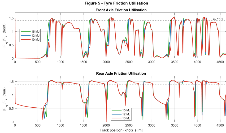
Figure 7.6: Tyre friction utilisation |F_{xy}|/F_z for front (top) and rear (bottom) axles vs. track position. The dashed line marks the nominal \mu_0 = 1.4 ; values above it are physically admissible due to load sensitivity.
