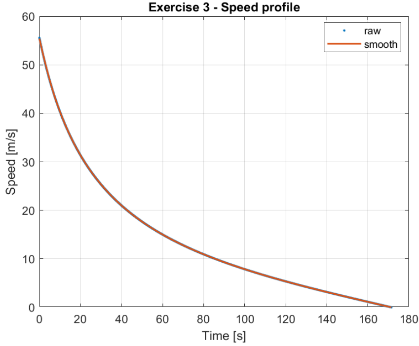
Figure 1.5: Measured coast-down speed profile, raw and after Savitzky–Golay smoothing.
