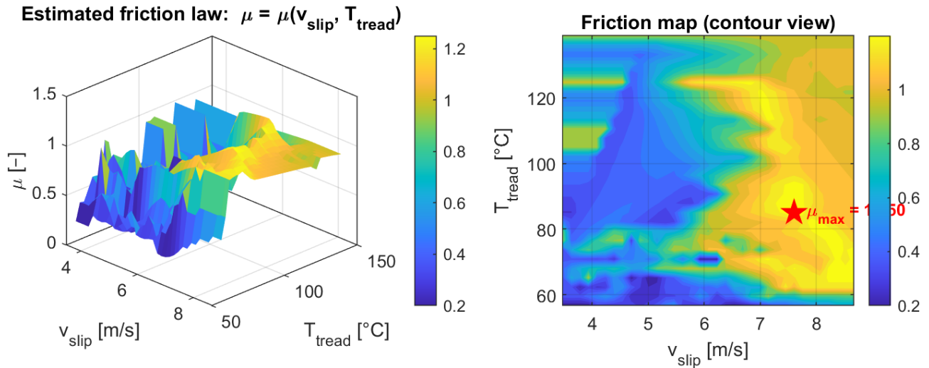
Figure 2.10: Estimated friction law surface (left) and contour map (right). The red star marks the maximum friction point.
