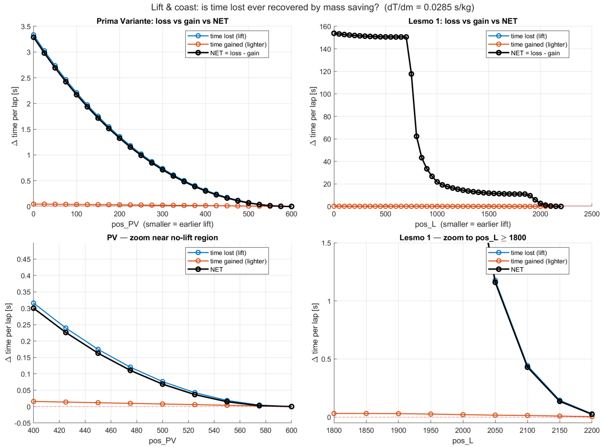
Figure 5.8: Per-corner decomposition: time lost by lifting (blue), time gained from the lighter average car (orange), and net per-lap delta (black). The red dashed line marks the break-even. None of the explored points crosses below zero , i.e. the mass saving never pays back the time directly lost in the lift window. Top row: full range. Bottom row: zoom around the no-lift region.
