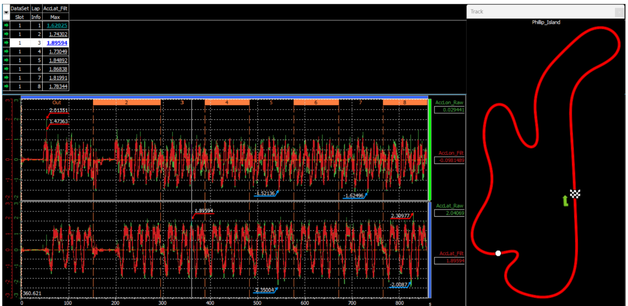
Figure 6.5: Lap report on the lateral acceleration channel for lap 3
