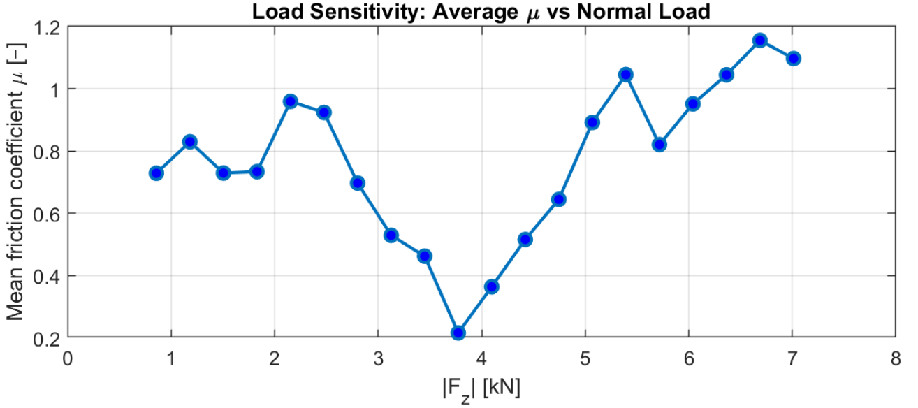
Figure 2.13: Mean friction coefficient as a function of normal load |F_z| .
