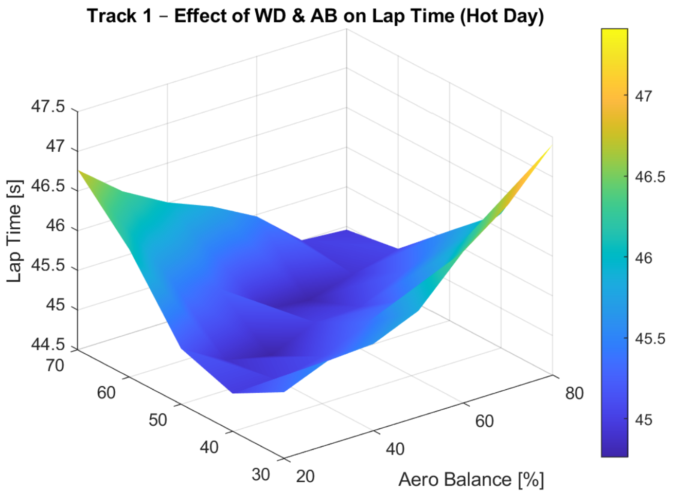
Figure 2.5: Average lap time surface as a function of weight distribution (WD) and aerodynamic balance (AB) on Track 1, Hot Day conditions.
