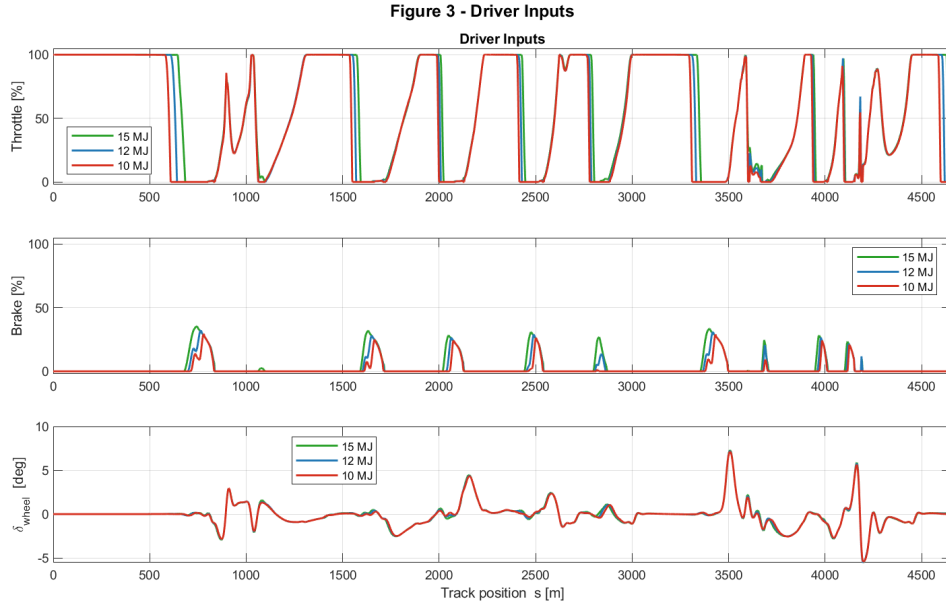
Figure 7.4: Normalised throttle (%), brake (%), and road-wheel steering angle ( ^{\circ} ) vs. track position for the three energy budgets.
