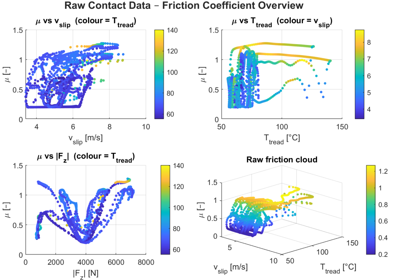
Figure 2.9: Raw friction data overview. Top-left: \mu vs. slip speed (colour: T_{\text{tread}} ). Top-right: \mu vs. temperature (colour: v_{\text{slip}} ). Bottom-left: \mu vs. normal load. Bottom-right: 3-D scatter cloud.
