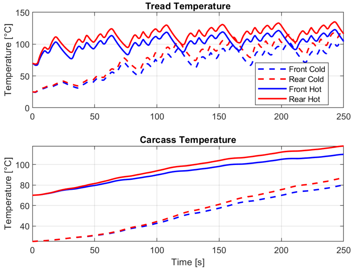
Figure 2.3: Tread and carcass temperature evolution for the reference case ( \delta_{\text{toe}} = 0 ) under Cold Night (dashed) and Hot Day (solid) conditions. Front tyres in blue, rear in red.
