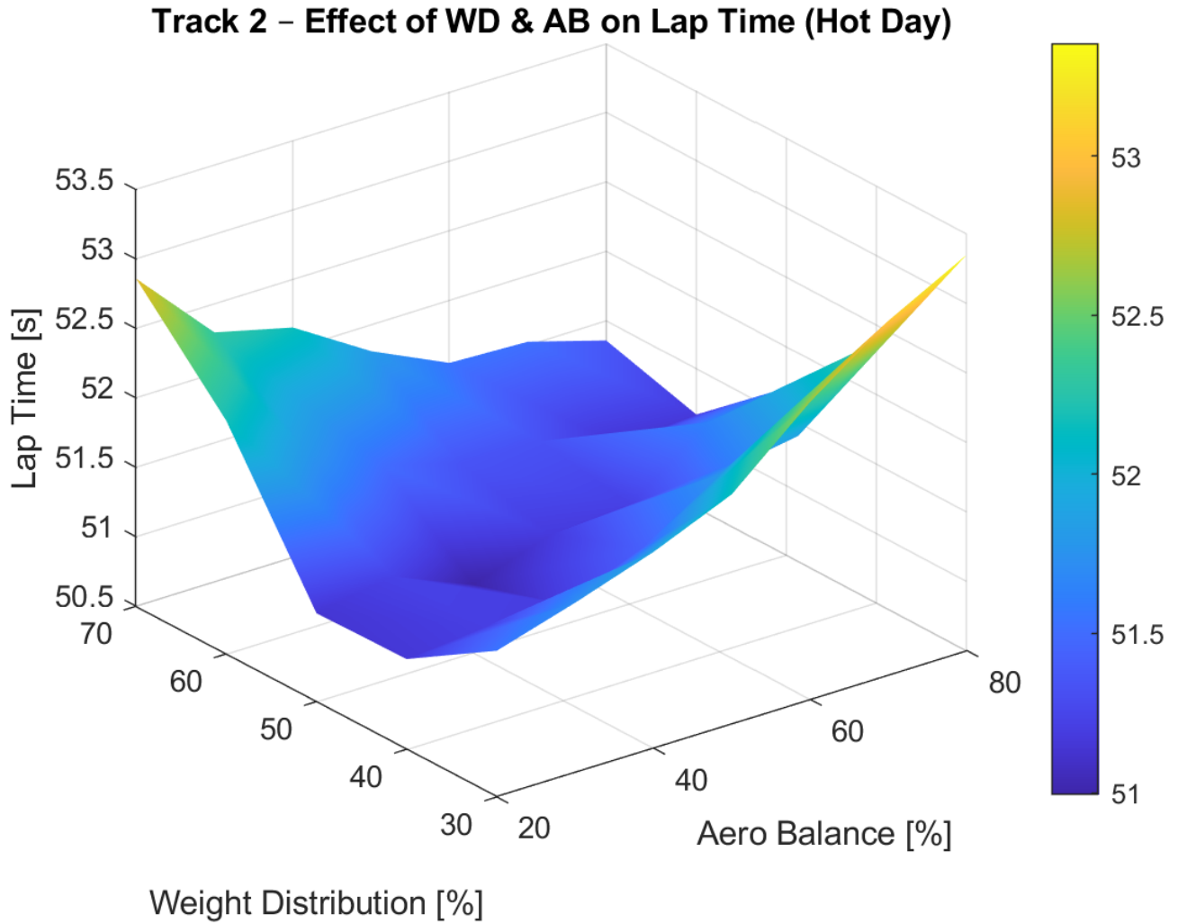
Figure 2.6: Average lap time surface as a function of WD and AB on Track 2, Hot Day conditions.
