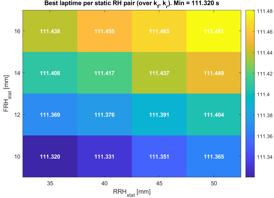
Figure 5.2: Best laptime per (\text{FRH}_{\text{stat}}, \text{RRH}_{\text{stat}}) pair (i.e. minimum over the 4 \times 4 stiffness combinations).
