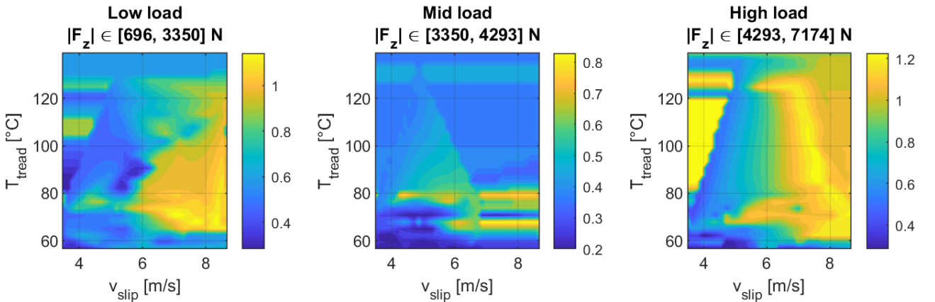
Figure 2.12: Friction maps for three normal-load bands: low (left), mid (centre) and high (right).
