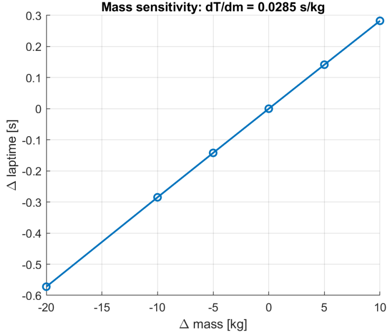
Figure 5.4: Lap time delta as a function of vehicle mass perturbation around the 605 kg baseline. The slope is \partial T/\partial m = 0.0285 \text{ s/kg} .
