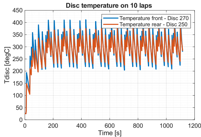
Figure 4.2: Thermal analysis on a 10 lap segment for the selected pair of discs
