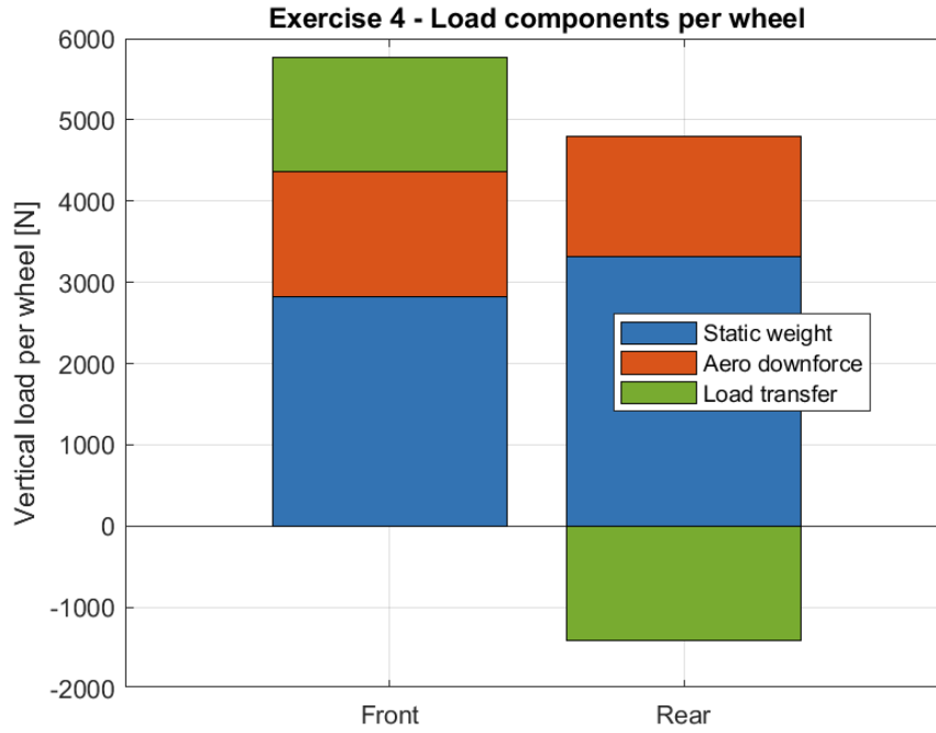
Figure 1.7: Decomposition of vertical load per wheel into static weight, aerodynamic downforce, and longitudinal load transfer. The load transfer increases the front load and reduces the rear.
