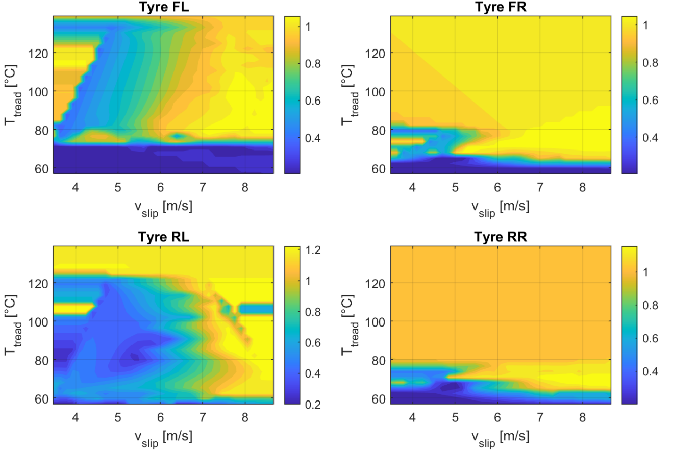
Figure 2.11: Individual friction maps for the four tyres (FL, FR, RL, RR). Differences reflect asymmetric loading due to the specific lap trajectory.
