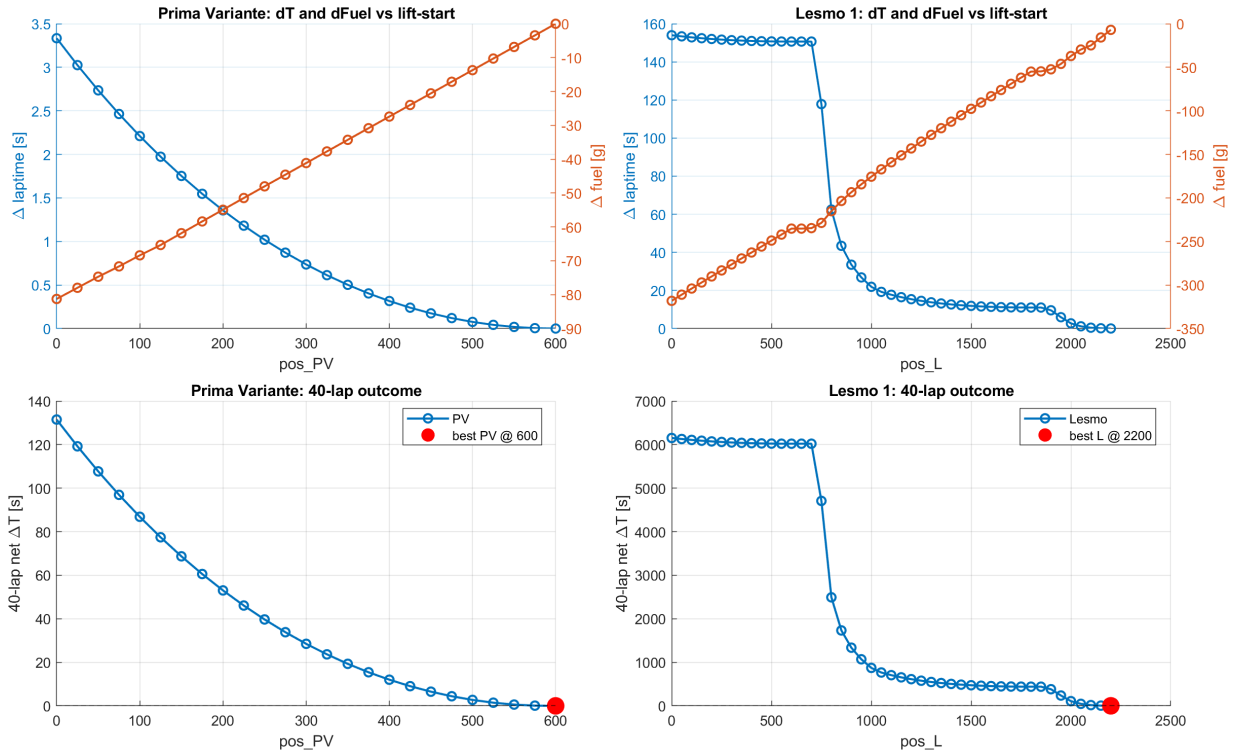
Figure 5.7: Per-corner sweep summary: top row shows \Delta T and \Delta fuel as a function of lift-start position; bottom row shows the 40-lap net \Delta T outcome. The red marker highlights the best (least bad) lift-start position from a pure laptime perspective.
