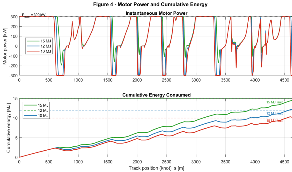
Figure 7.5: Instantaneous motor power (top) and cumulative energy consumption (bottom) vs. track position. Dashed horizontal lines mark the energy limits; the dotted line marks P_{\max} = 300 \text{ kW} .
