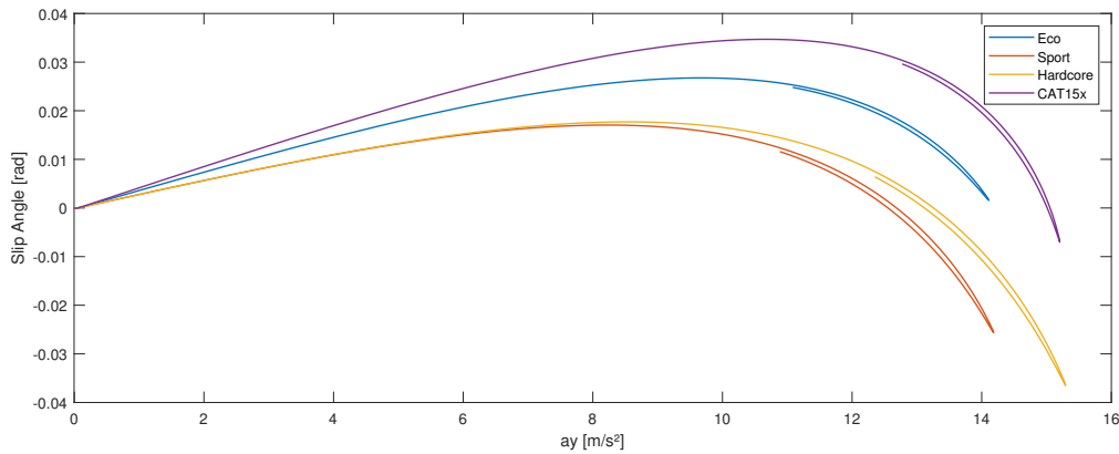
Figure 5.3: a_y vs \beta for the different modes.
