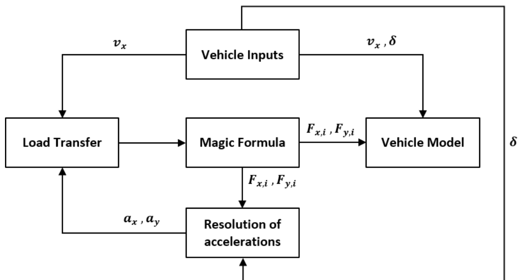
Figure 4.3: Diagram Dual Track Model.
