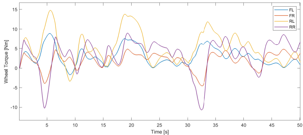
Figure 7.10: AutoX Torques Results.
