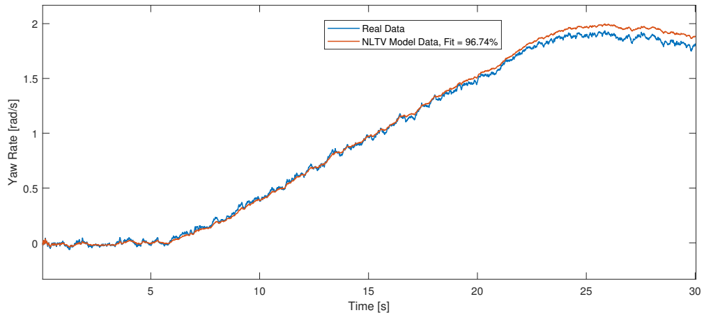
Figure 4.4: Comparison between NLTV Model and CAT15x Data on a Ramp Steer.
