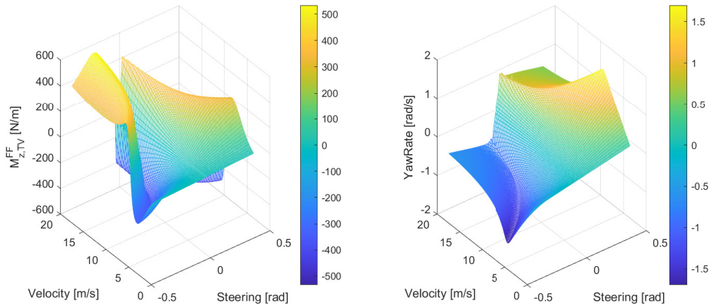
Figure 5.4: v_x vs \delta vs M_{z,TV}^{FF} and \dot{\psi}_{ref} on Sport mode.
