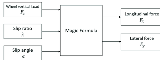
Figure 3.7: Inputs and outputs from a simplified Magic Formula.
