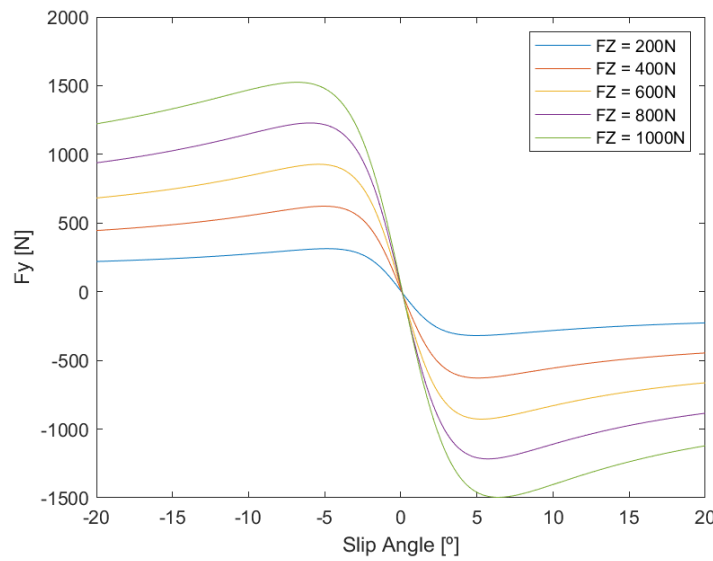
Figure 3.11: Fy vs Slip Angle.
