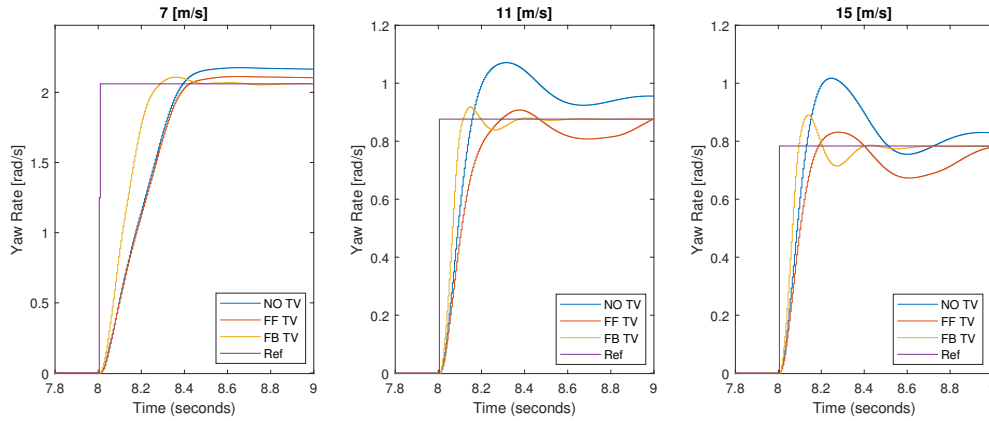
Figure 5.5: Step Steer response for different controllers and velocities.
