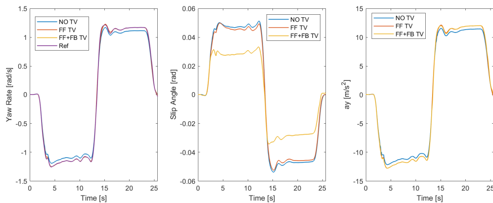
Figure 7.2: Skid Pad Vehicle Behaviour Results.
