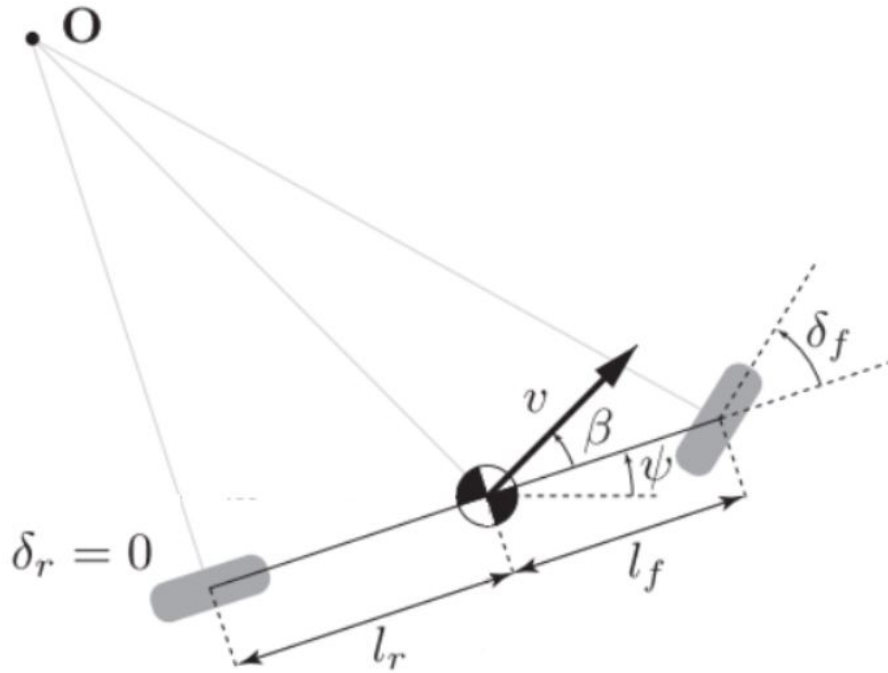
Figure 4.1: Bicycle Model Scheme Representation.
