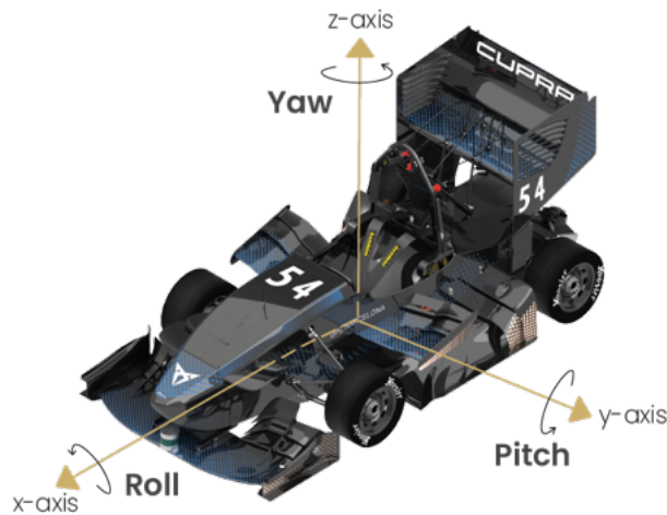
Figure 3.1: Vehicle Reference Axis.
