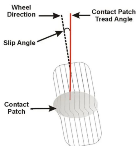
Figure 3.10: Slip Angle Scheme.
