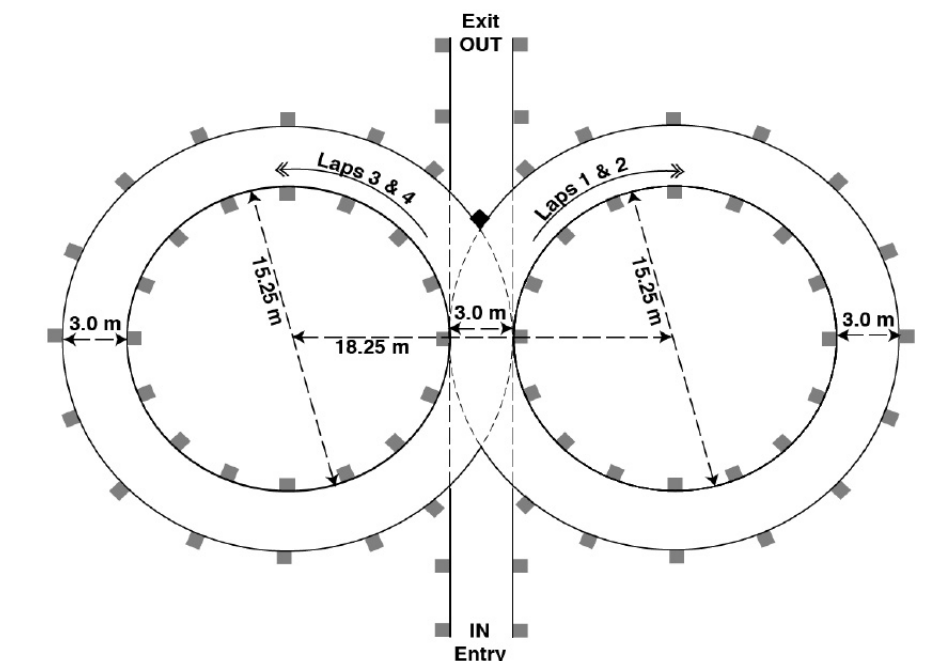
Figure 2.4: Skid-Pad track scheme.
