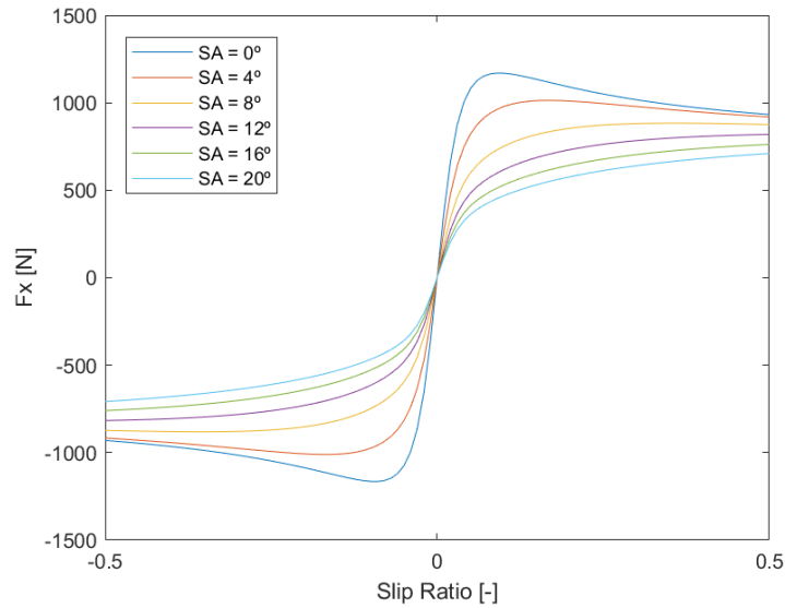
Figure 3.12: F_x vs Slip Ratio vs Slip Angle.
