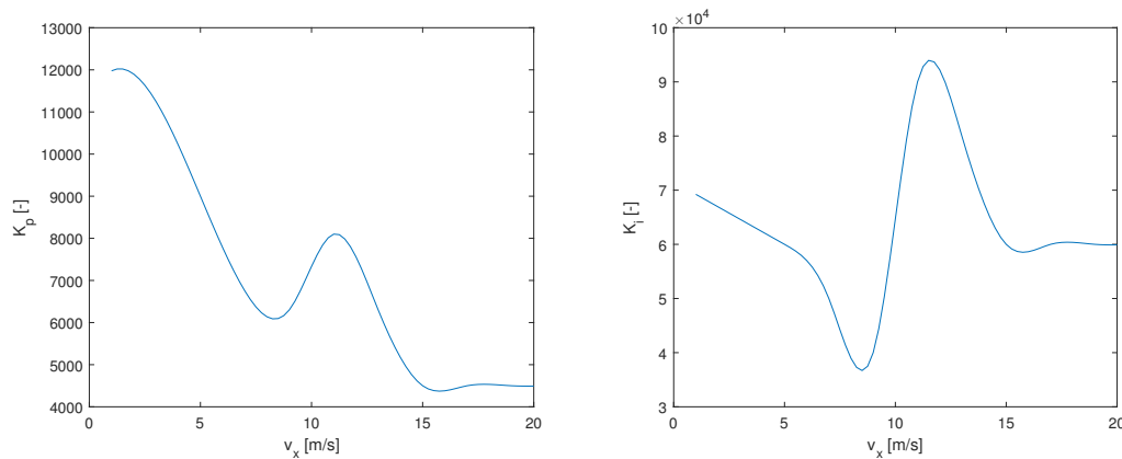
Figure 5.6: K_p and K_i plot.
