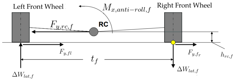
Figure 3.4: Lateral transfer load using roll motion.
