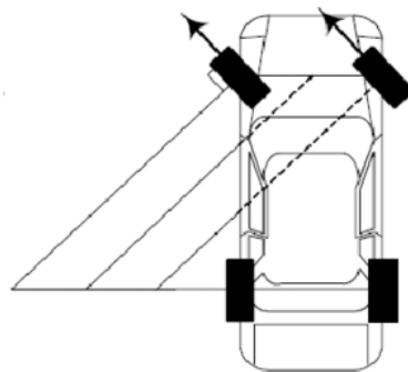
Figure 3.15: Parallel Steering System.
