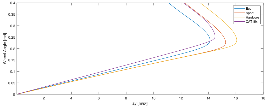
Figure 5.2: a_y vs \delta for the different modes.
