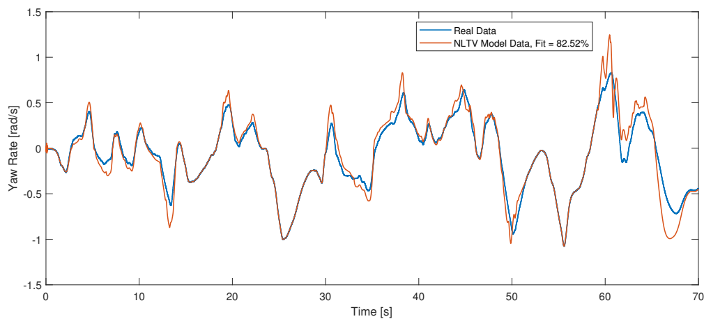
Figure 4.6: Comparison between NLTV Model and CAT15x Data on the FSS AutoX 2023.
