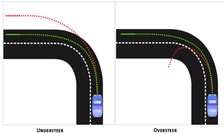
Figure 3.17: Understeer and Oversteer representation.
