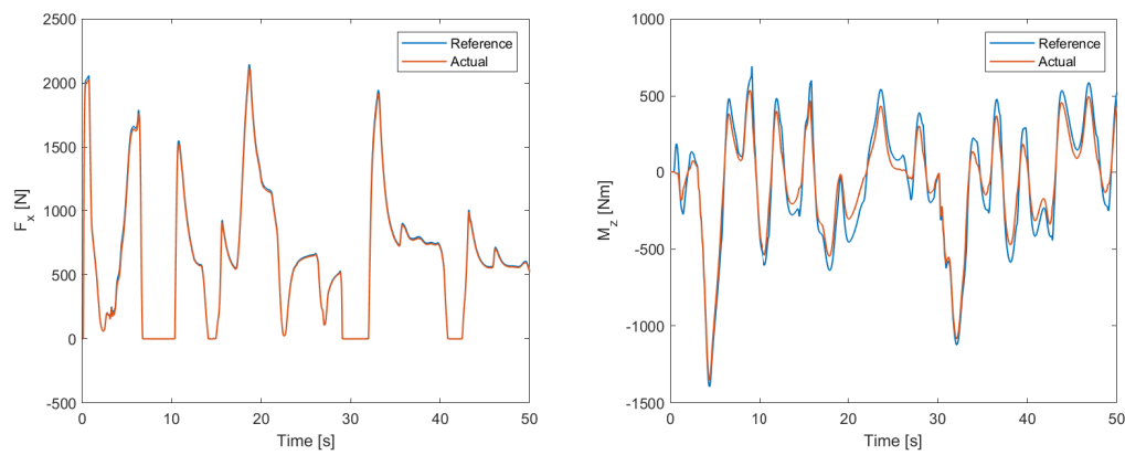
Figure 7.9: SkidPad Torque Distribution Objectives Results.
