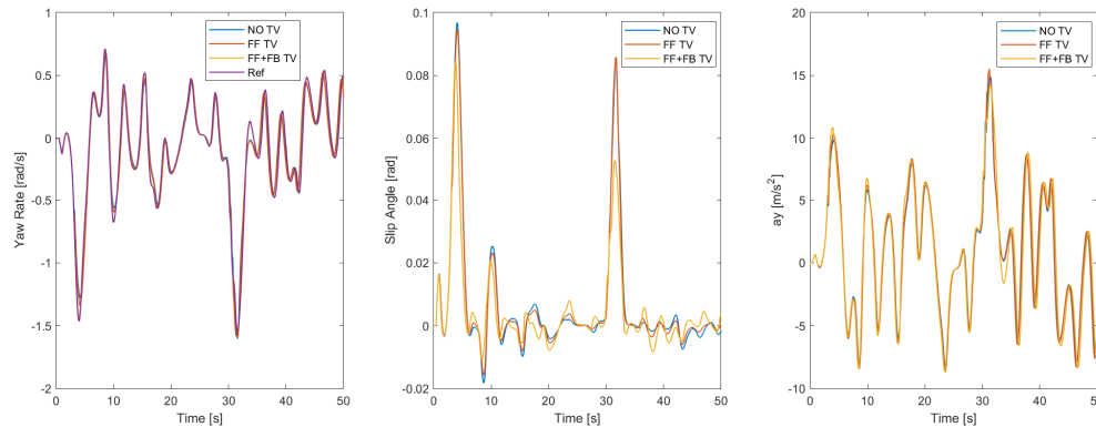
Figure 7.3: AutoX Vehicle Behaviour Results.
