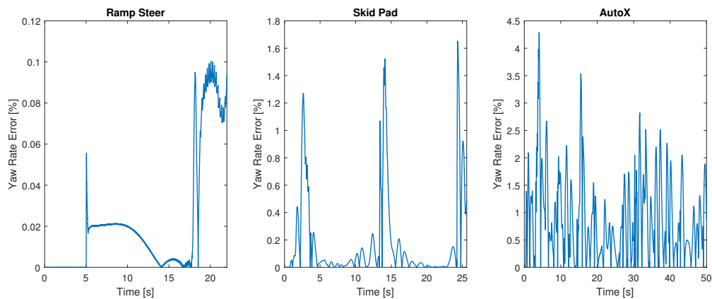
Figure 7.4: Error between actual and reference yaw rate.
