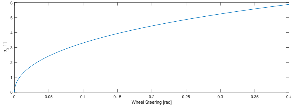
Figure 6.5: \alpha_2 priority coefficient splie.
