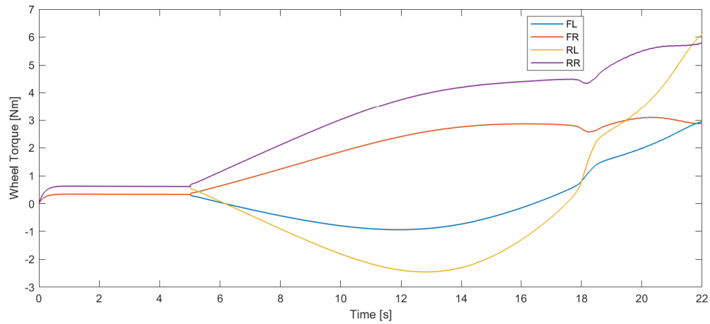
Figure 7.6: Ramp Steer Torques Results.
