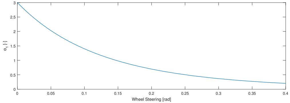
Figure 6.4: \alpha_1 priority coefficient splie.
