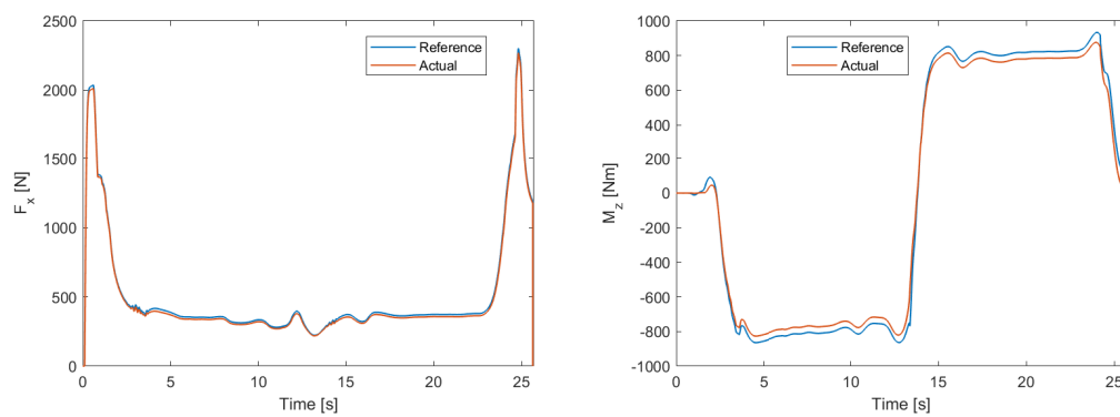
Figure 7.7: Skid Pad Torque Distribution Objectives Results.
