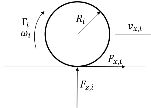
Figure 3.8: Slip Ratio Scheme.
