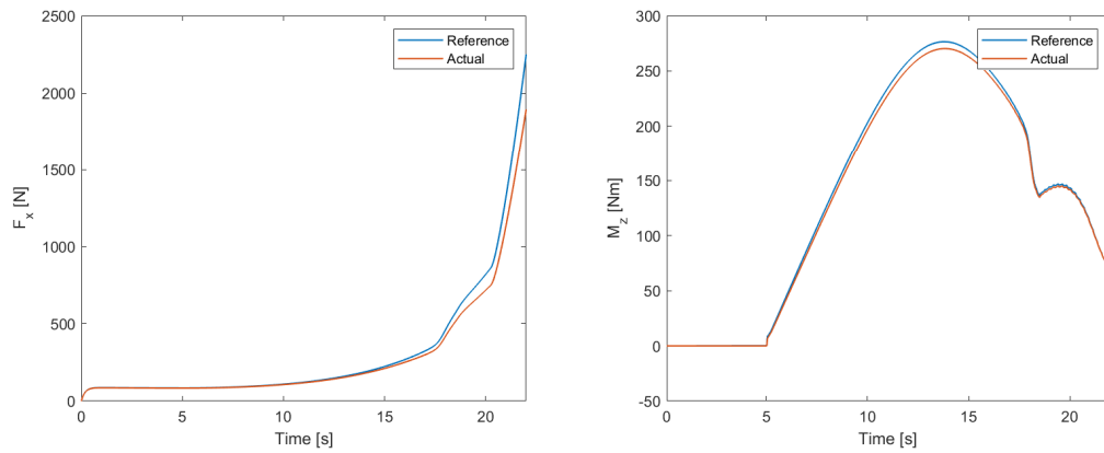
Figure 7.5: Ramp Steer Torque Distribution Objectives Results.
