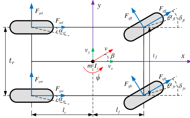
Figure 6.2: 4WD Vehicle Dynamics Model.
