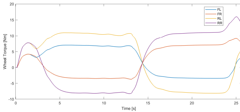
Figure 7.8: Skid Pad Torques Results.
