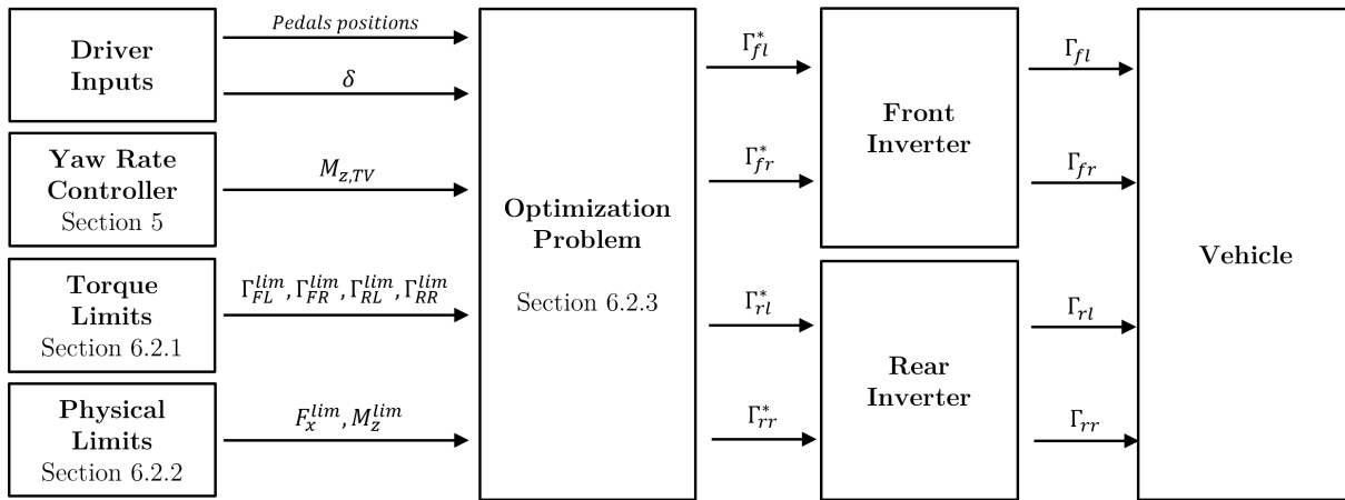
Figure 6.1: Torque Allocator Scheme.
