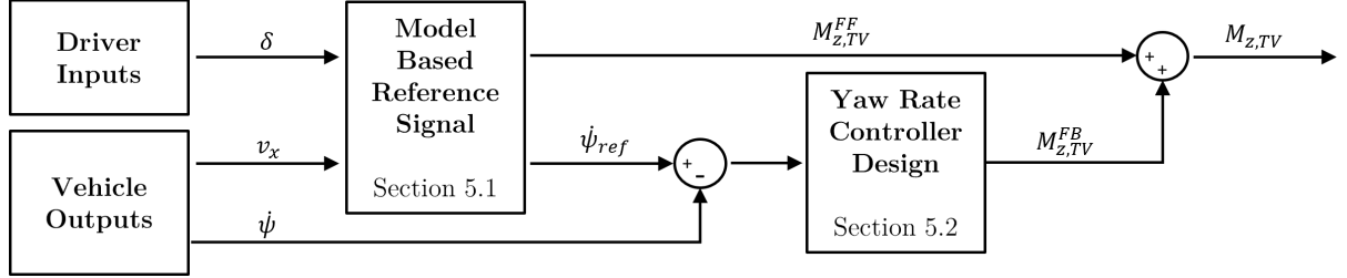
Figure 5.1: Yaw Rate Control Scheme.
