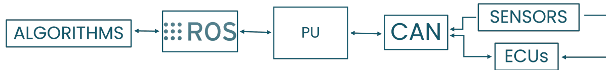
Figure 3.18: Car communication scheme.
