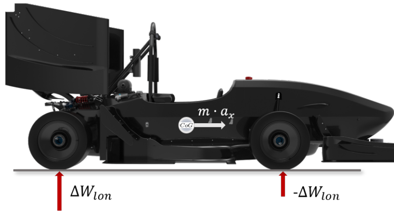
Figure 3.2: Longitudinal load transfer.
