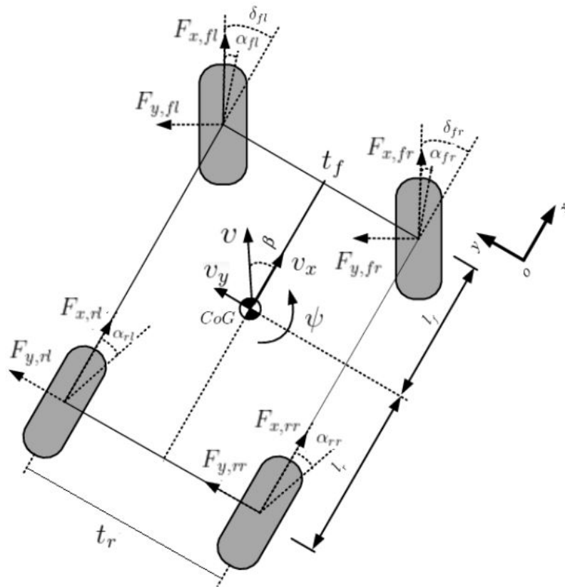
Figure 4.2: DualTrack Model Scheme Representation.
