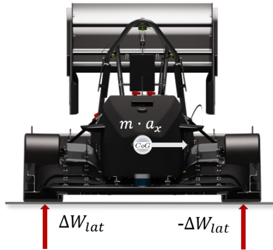
Figure 3.3: Lateral load transfer.
