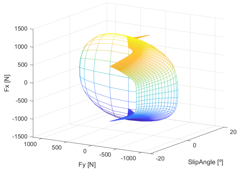
Figure 3.14: Friction Circle.
