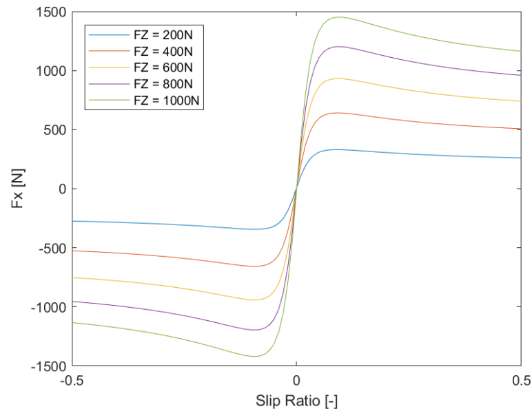
Figure 3.9: F_x vs Slip Ratio.
