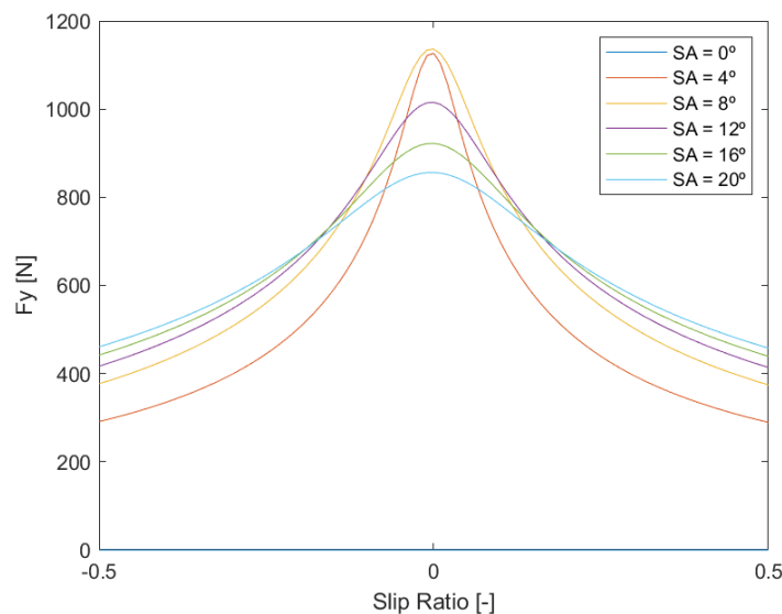
Figure 3.13: F_y vs Slip Ratio vs Slip Angle.
