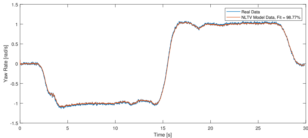
Figure 4.5: Comparison between NLTV Model and CAT15x Data on a Skid Pad.
