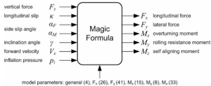
Figure 3.6: Inputs and outputs from Magic Formula.
