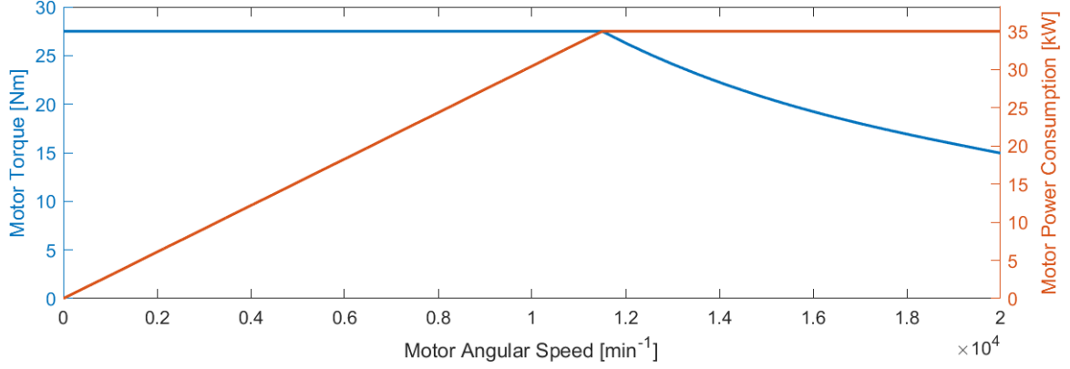
Figure 6.3: Torque motor spline. Angular speed vs Torque/Power consumption.
