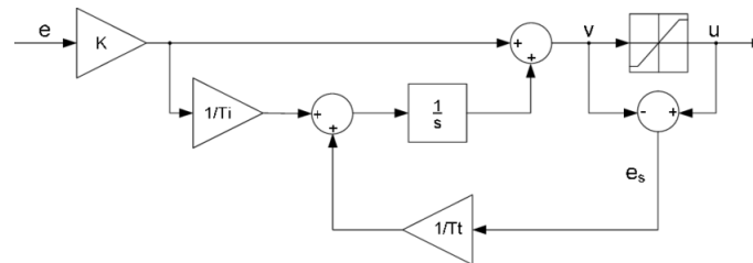
Figure 5.7: Back-calculation Antiwindup block diagram.
