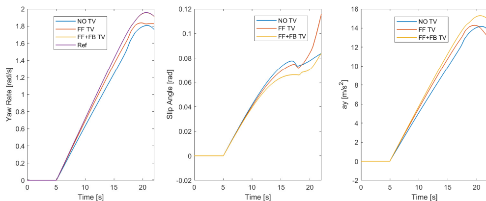
Figure 7.1: Ramp Steer Vehicle Behaviour Results.
