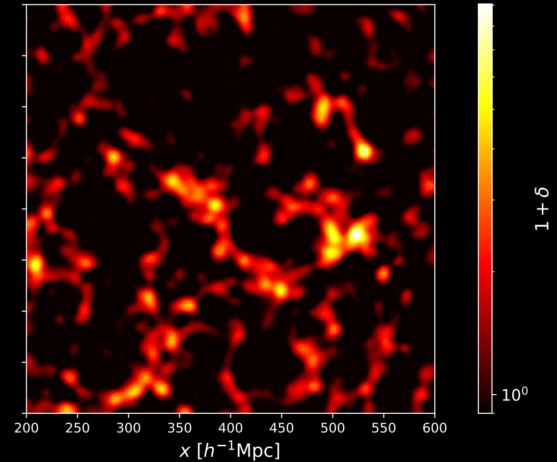
Corrected (Q)
