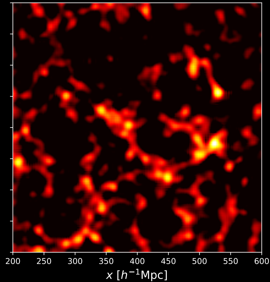
PM (initial)
