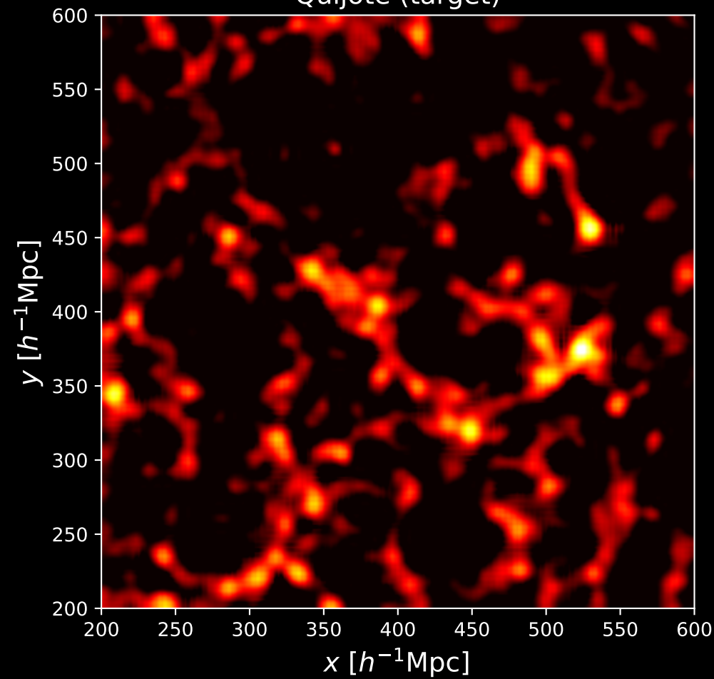
Quijote (target)
