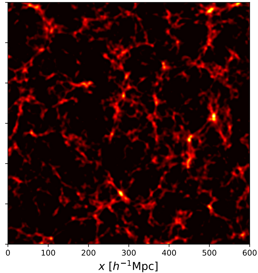
L-PICOLA (initial)
