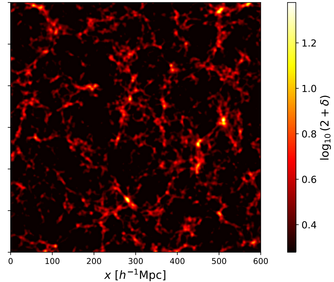
FastPM (initial)
