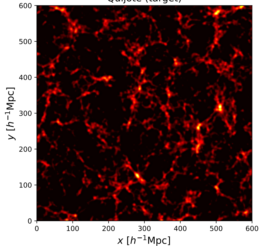
Quijote (target)
