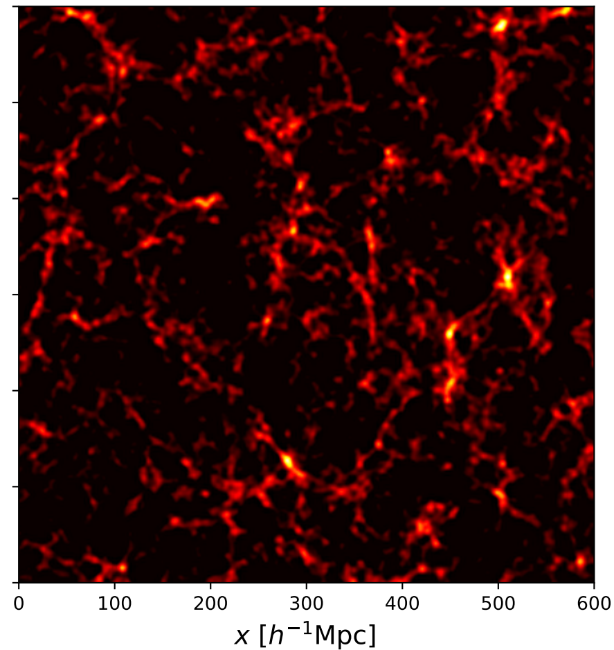
L-PICOLA (1 correction)
