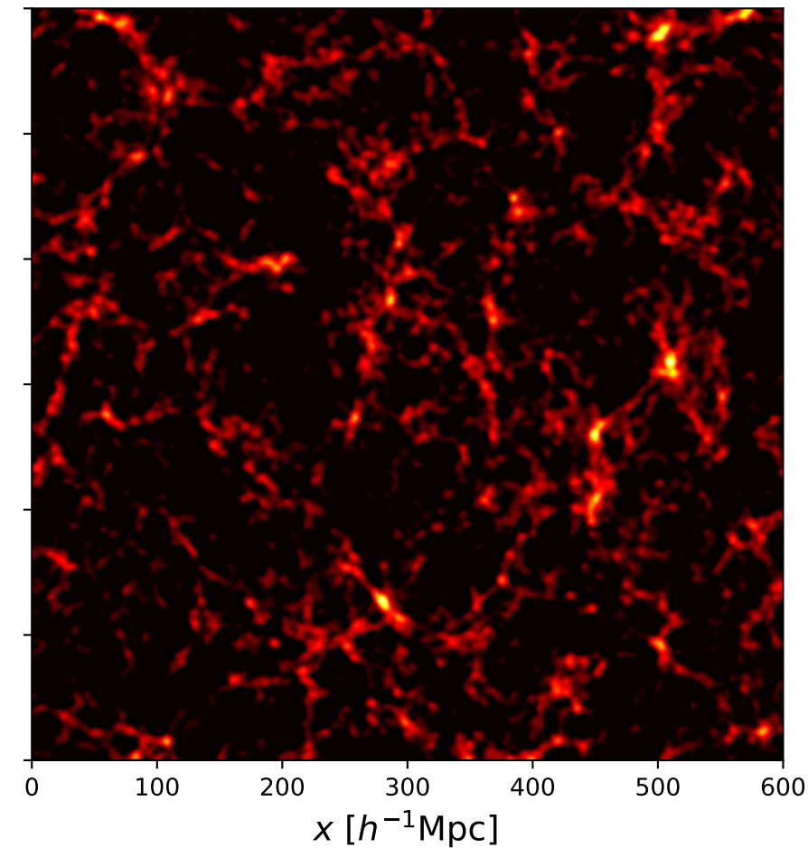
FastPM (1 correction)
