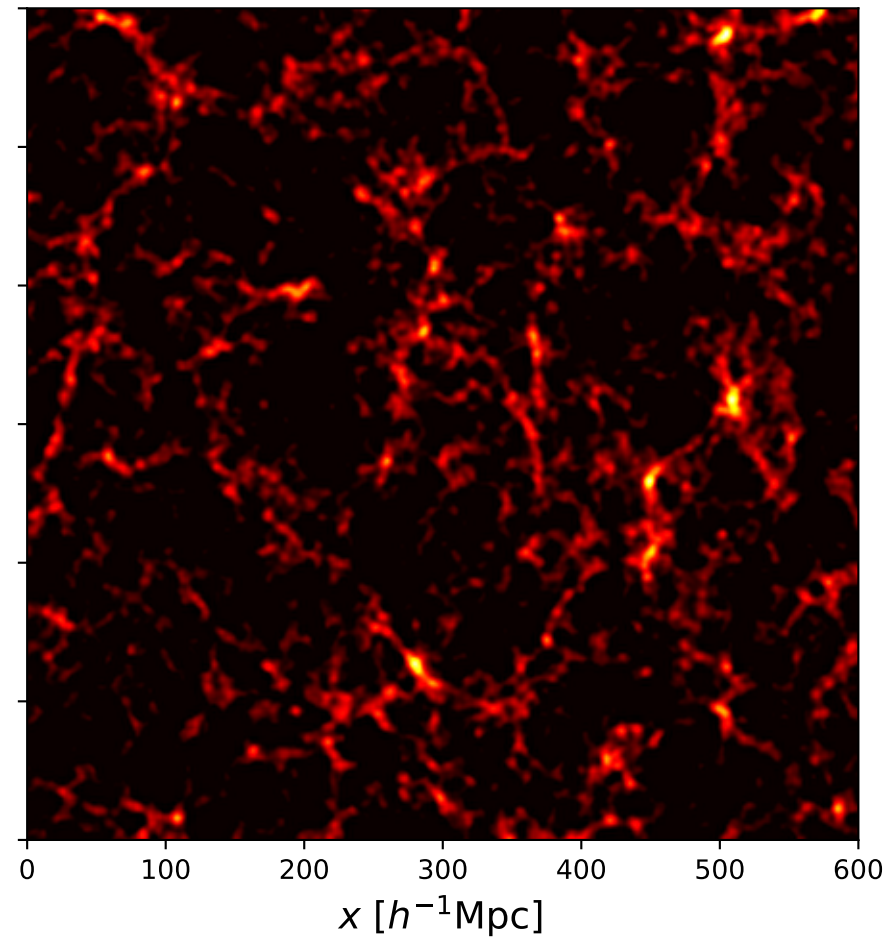
L-PICOLA (3 corrections)
