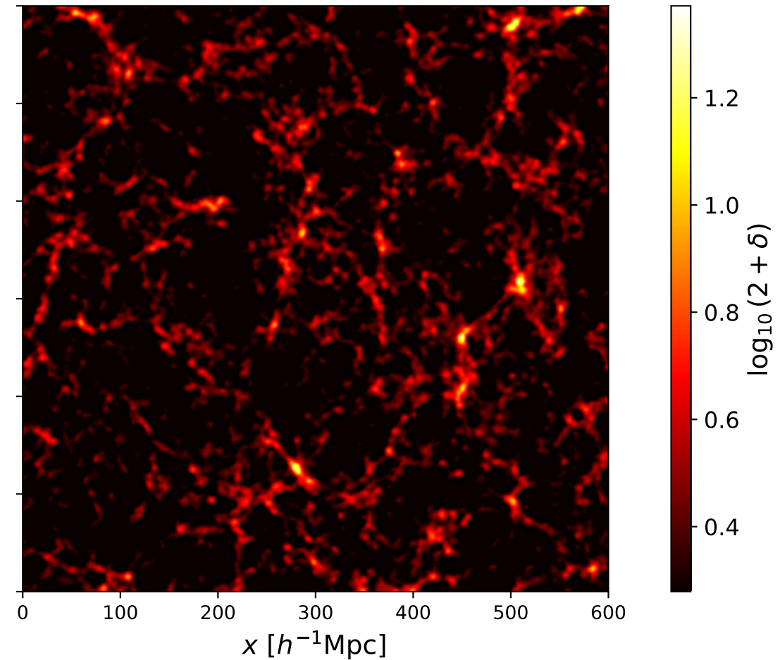
FastPM (3 corrections)
