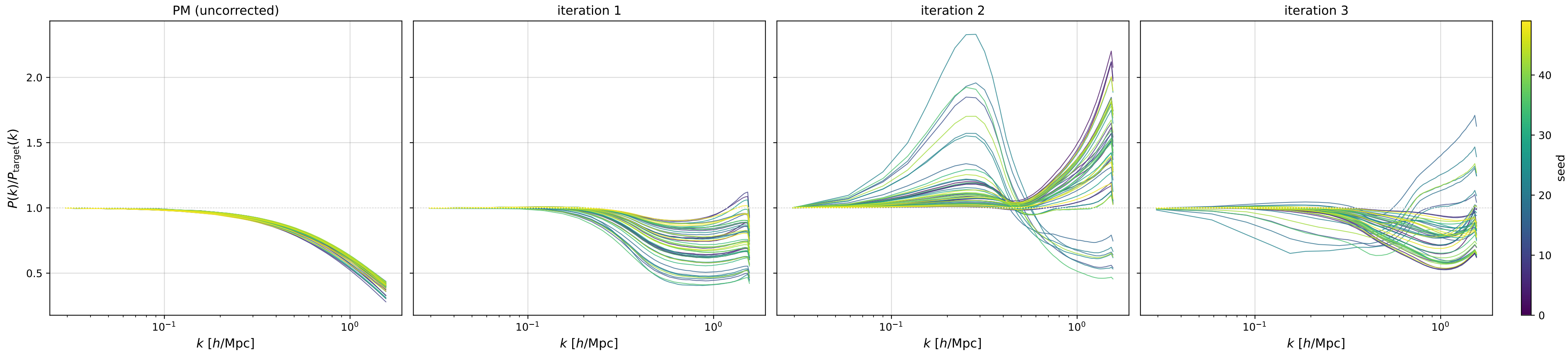
picola corr-case correction, lr = 0.50 ( N = 50 seeds)
