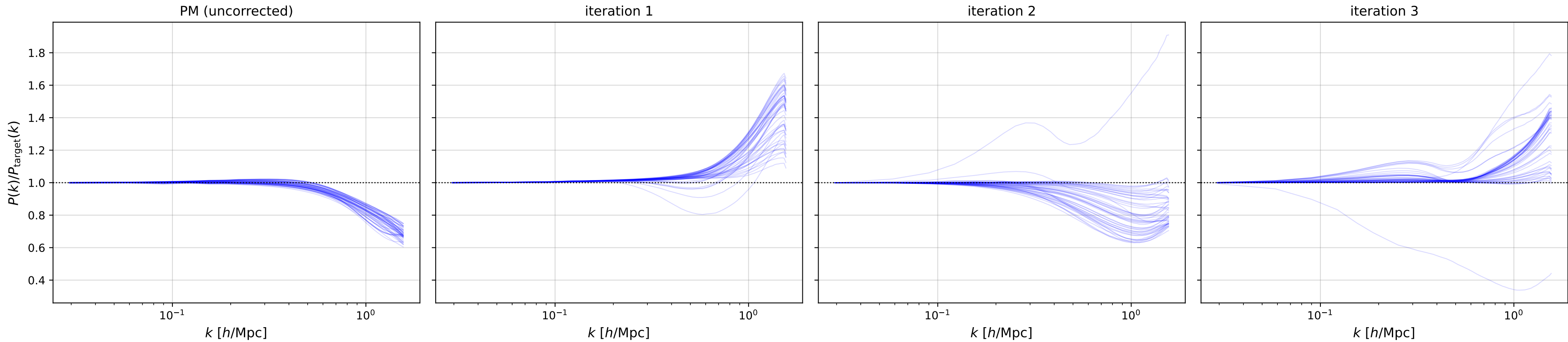
fastpm corr-case correction, \text{lr} = 0.30 ( N = 50 seeds)
