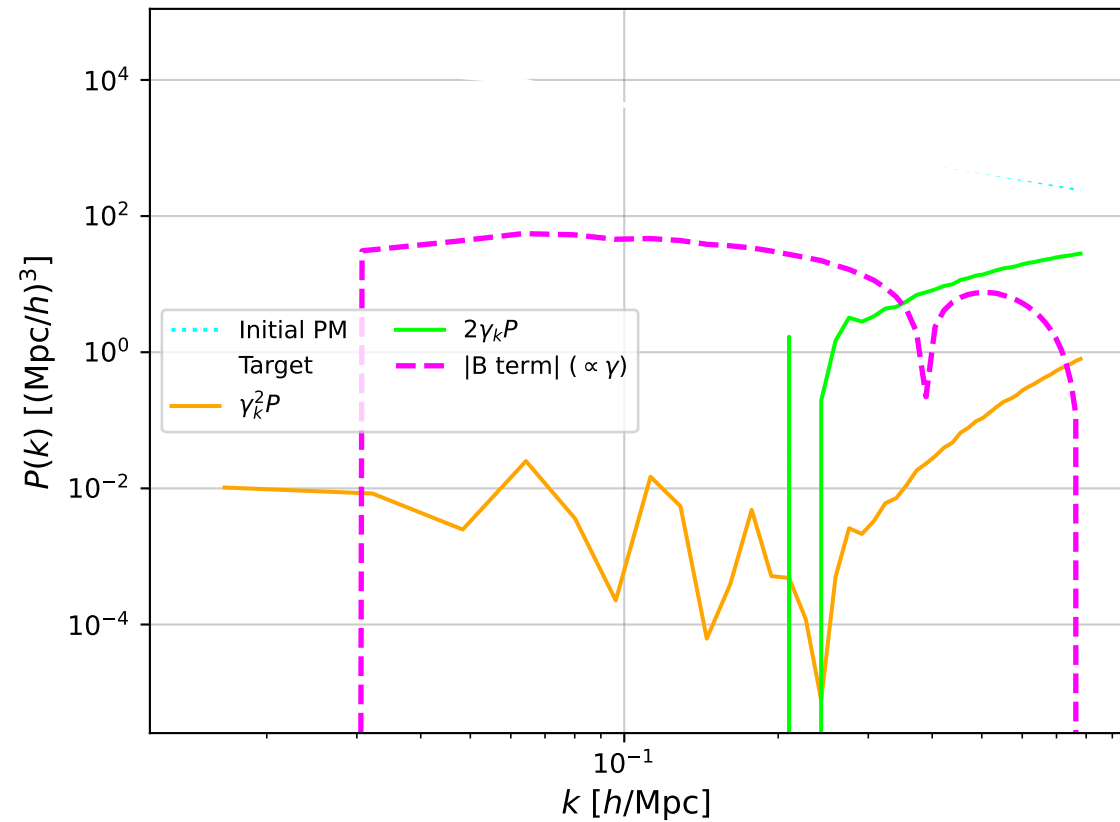
Bispectrum term contribution (using polynomial \gamma_k )
