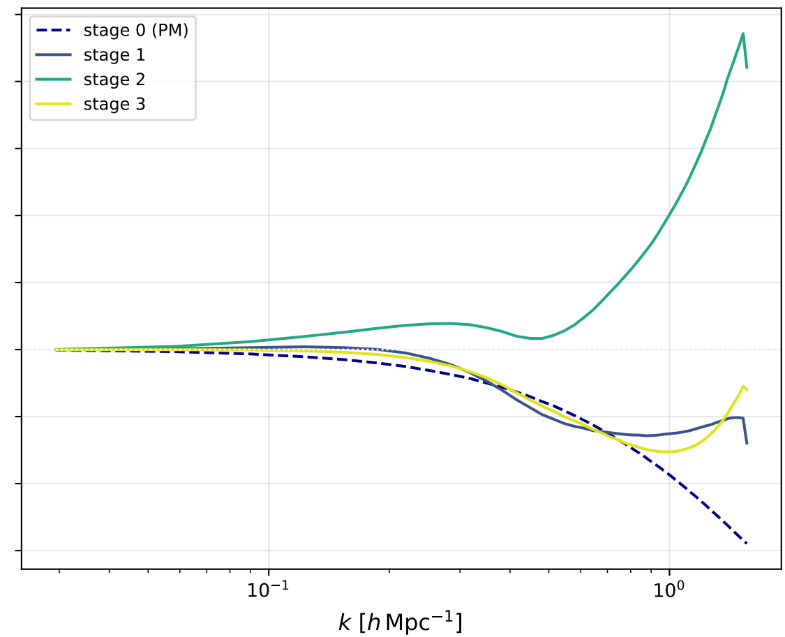
lr = 0.50
