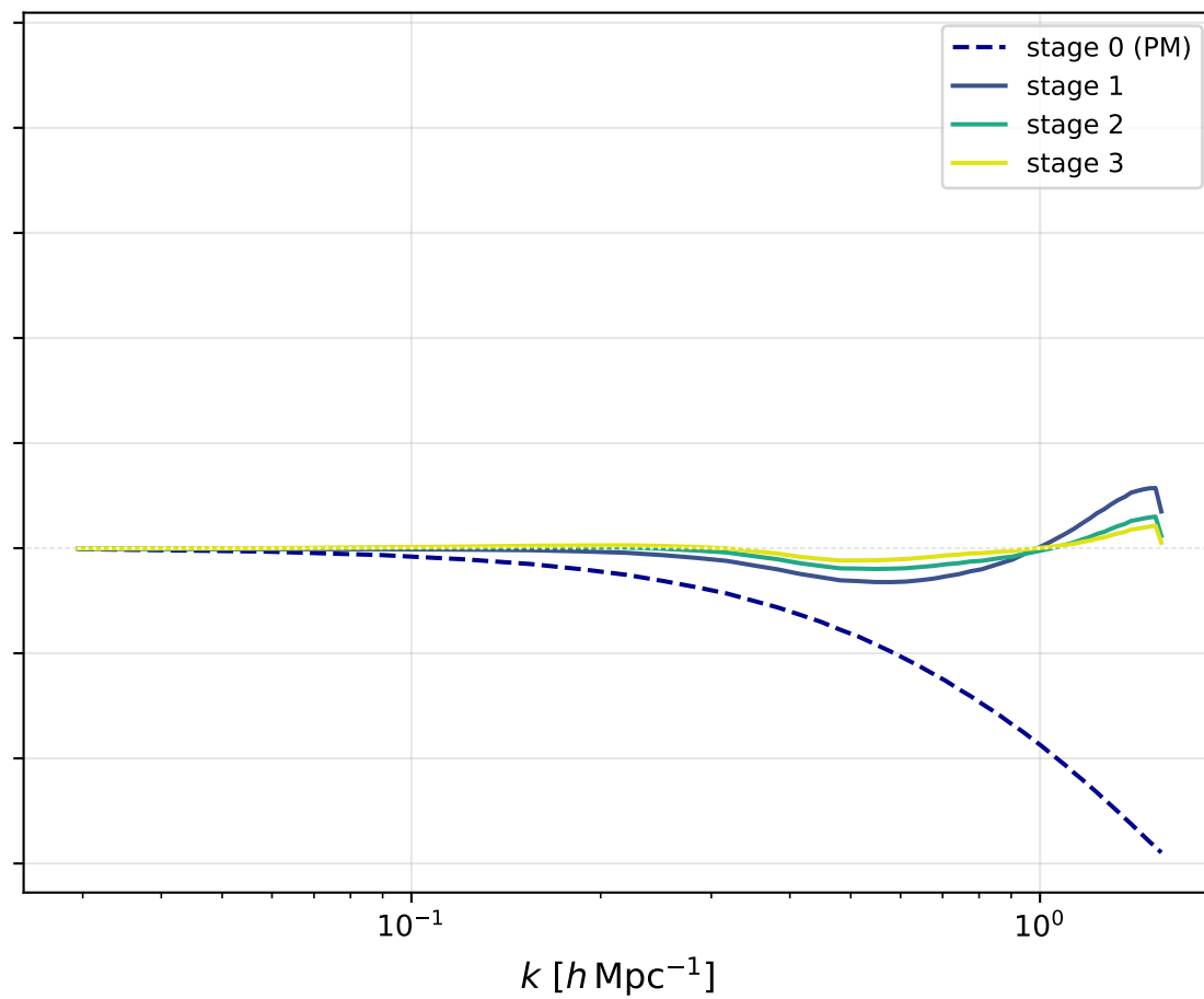
lr = 0.20
