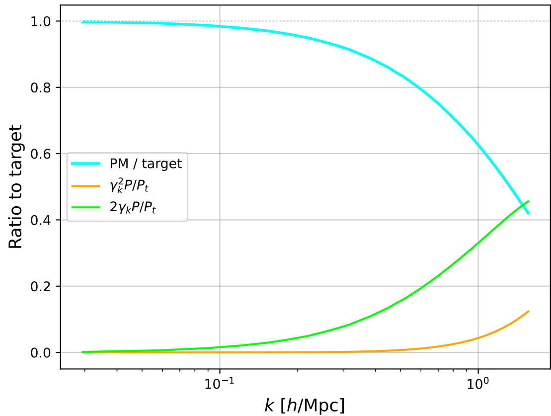
Correlated case — polynomial terms (no bispectrum)
