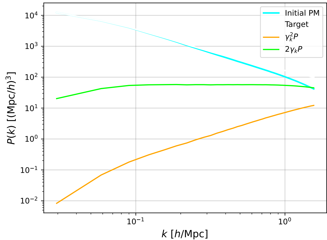
Correlated case — polynomial terms (no bispectrum)
