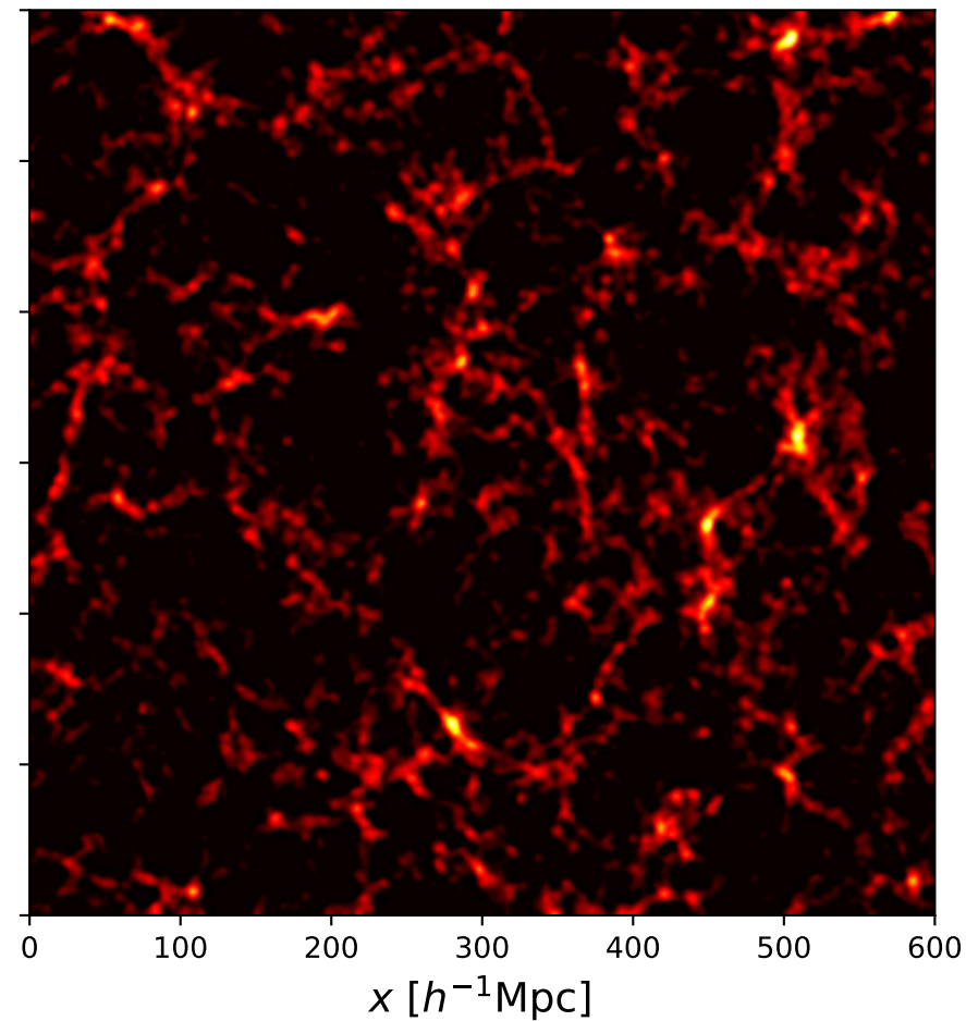
L-PICOLA (3 Q corrections)
