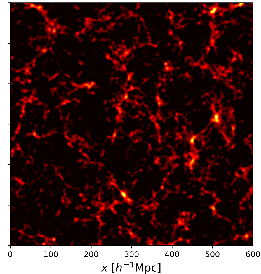
FastPM (3 Q corrections)
