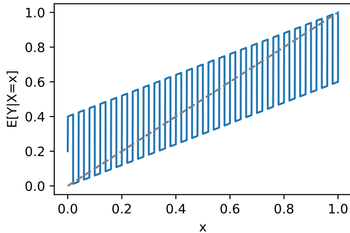
Conditional Probability
