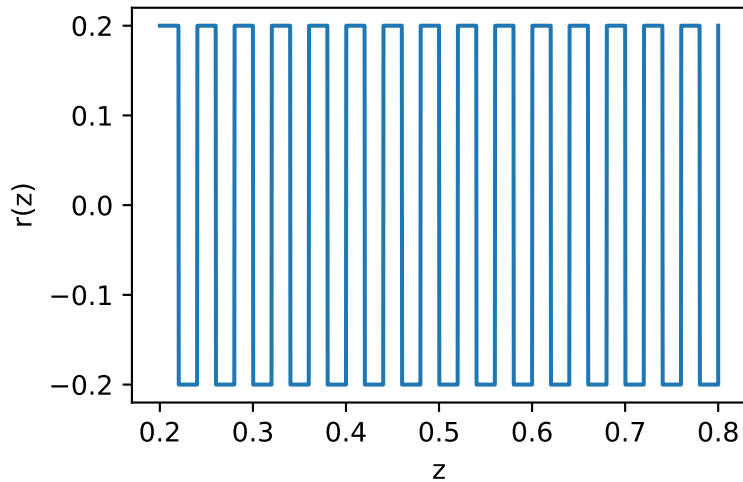
Residual Function
