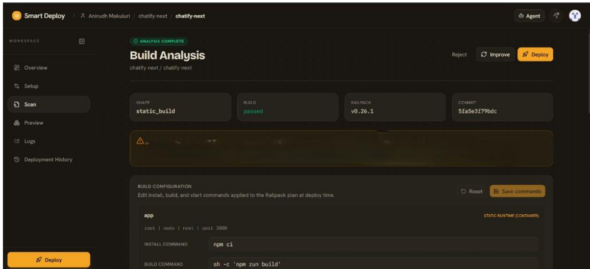
SmartDeploy Build Analysis — scan results with build validation, Railpack detection, and editable install/build commands
