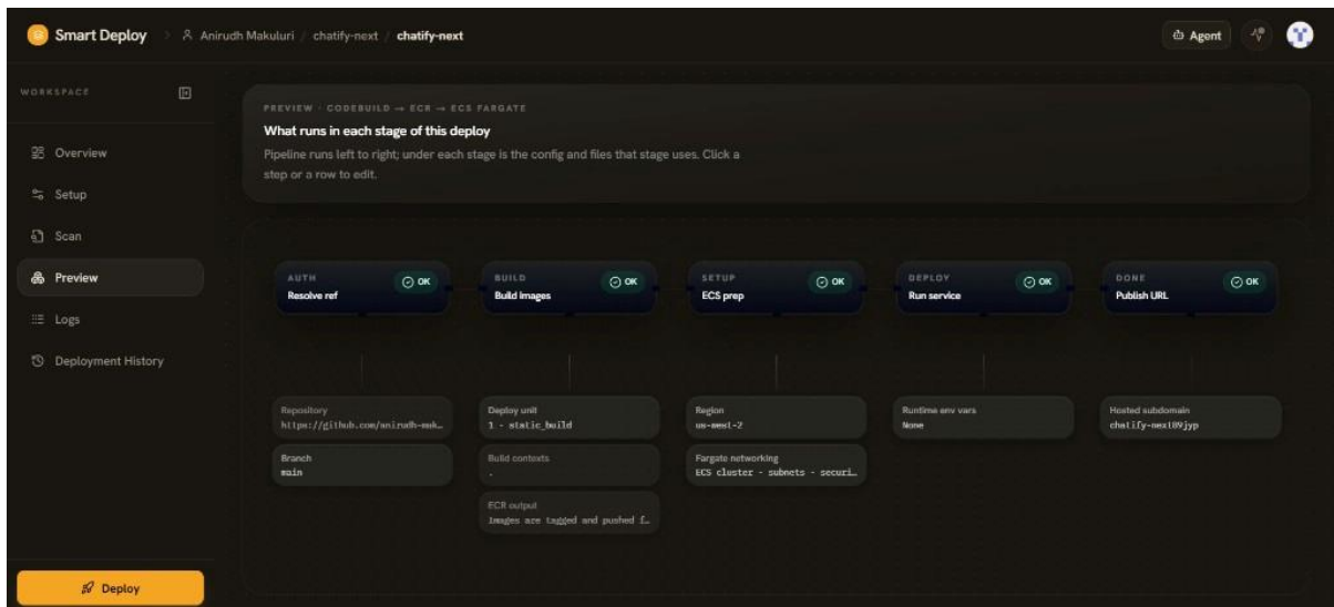
SmartDeploy Deployment Blueprint — preview of AUTH, BUILD, SETUP, DEPLOY, and DONE stages from GitHub to ECS Fargate
