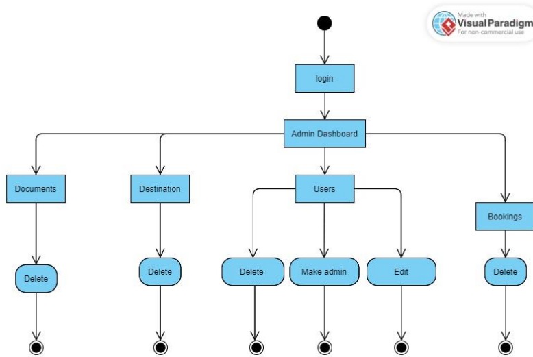
Figure 21: Activity Diagram of admin panel
