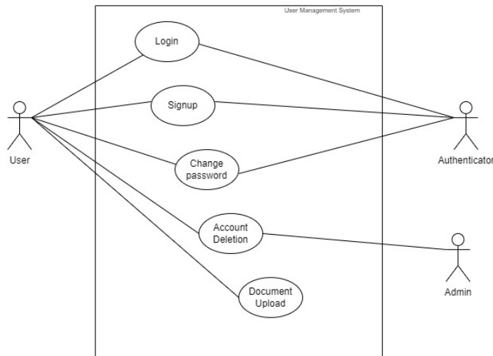
Figure 11: Use case diagram of user authentication
