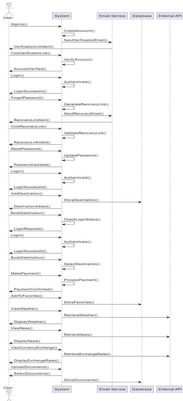
Figure 7: Sequence Diagram of TravelMate
