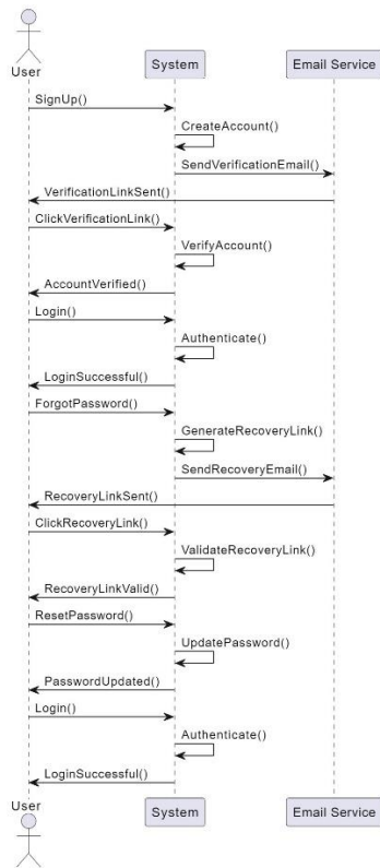
Figure 12: Sequence Diagram of user authentication system
