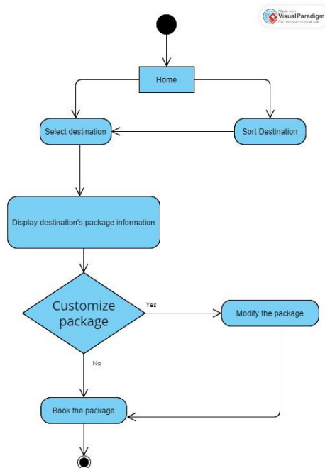
Figure 14: Activity Diagram of package booking system
