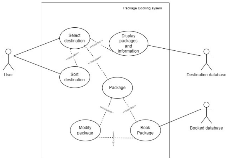
Figure 15: Use case diagram of package booking system
