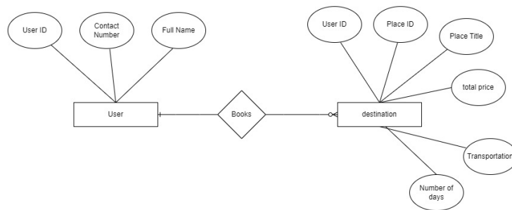
Figure 13: ERD Diagram of package booking
