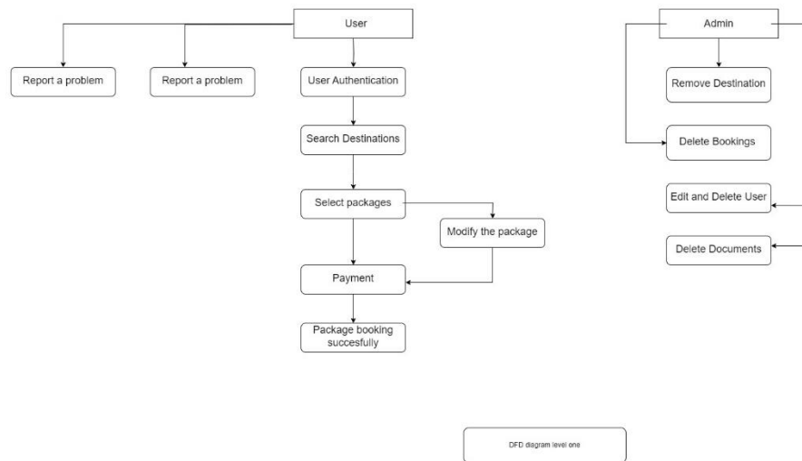
Figure 4: DFD Diagram level one
