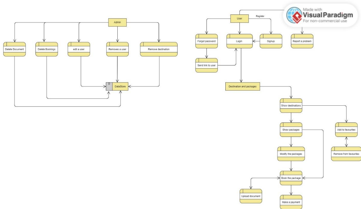
Figure 5: Level two DFD Diagram
