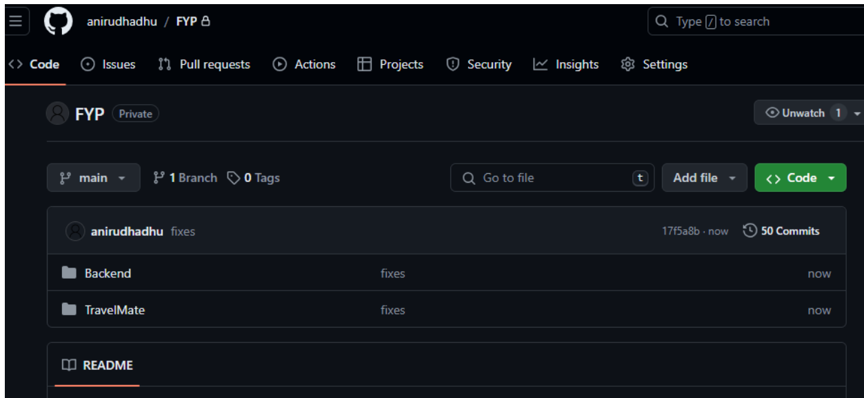
Figure 40: GitHub Commits
