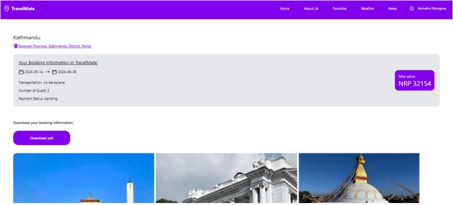
Figure 56: Booking page
