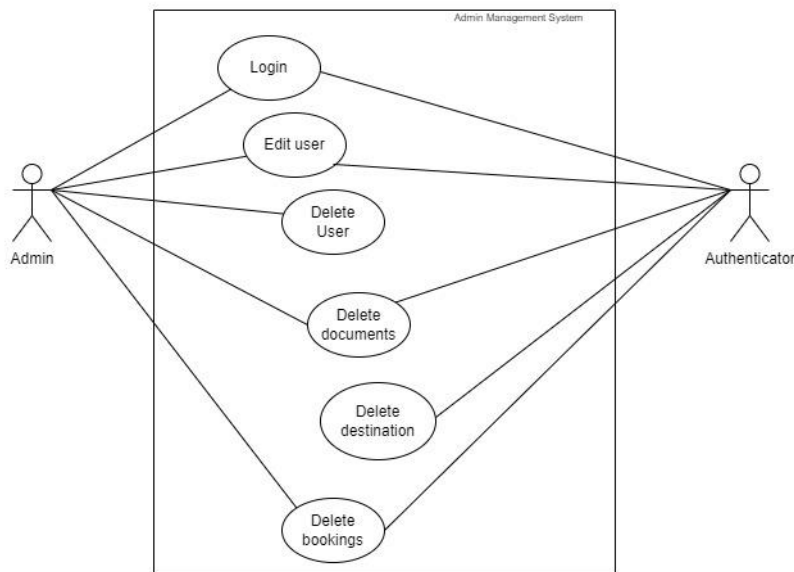
Figure 22: Use case diagram of admin panel
