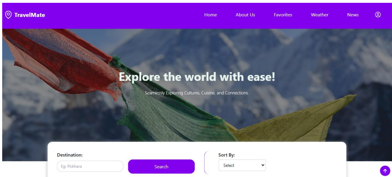
Figure 47: Landing page
