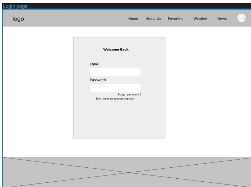
Figure 41: Login page
