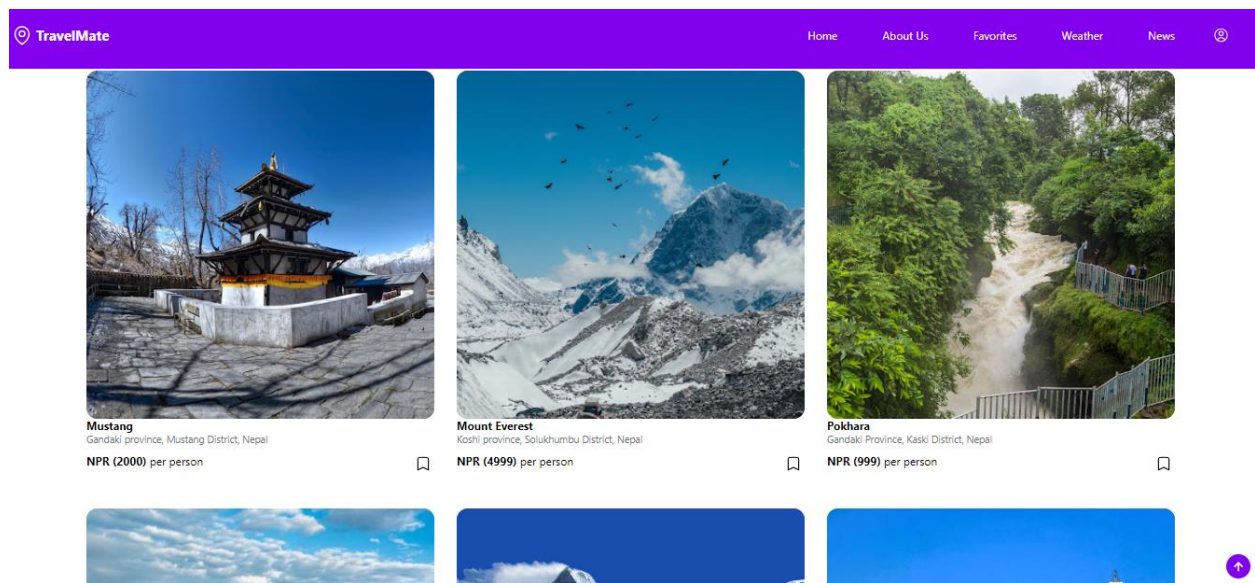
Figure 51: Destination Listing
