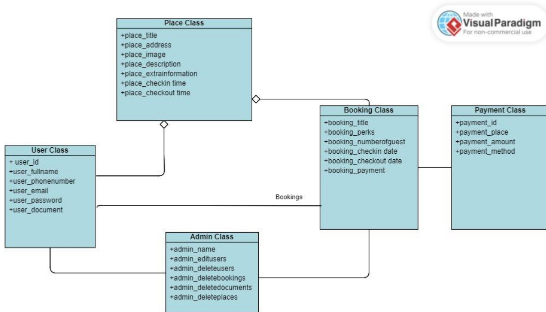
Figure 8: Class Diagram
