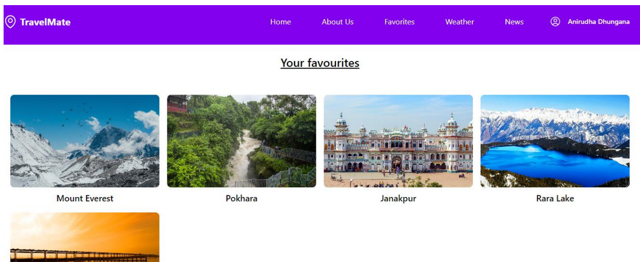
Figure 53: Favourites page
