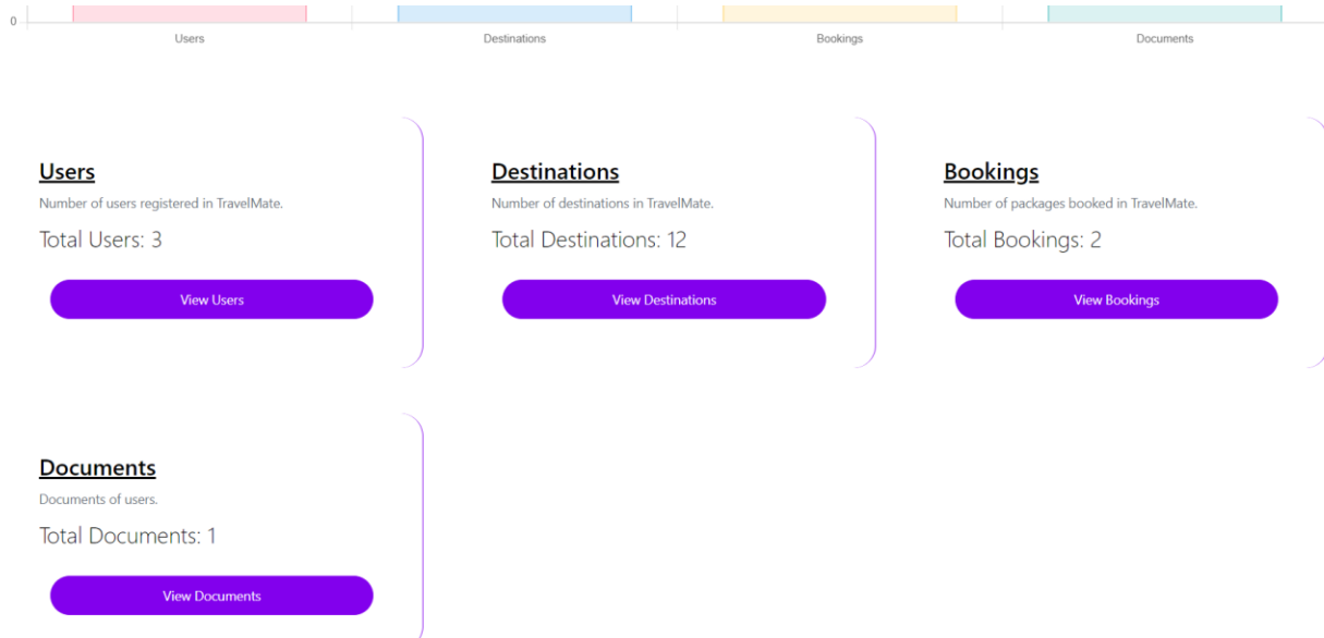
Figure 68: Admin dashboard 2
