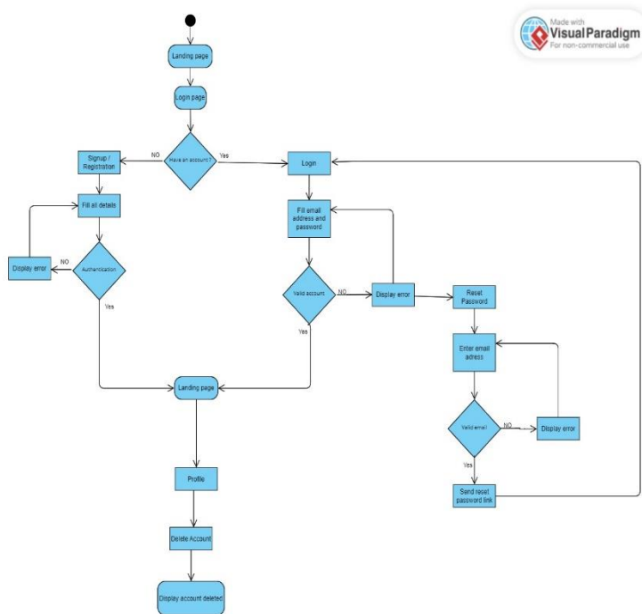
Figure 10: Activity Diagram of user authentication
