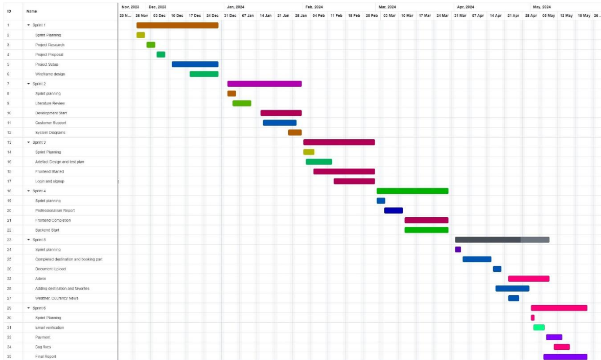
Figure 39: Gantt chart
