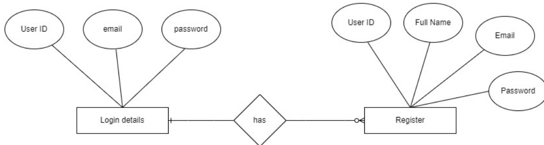
Figure 9: ERD diagram
