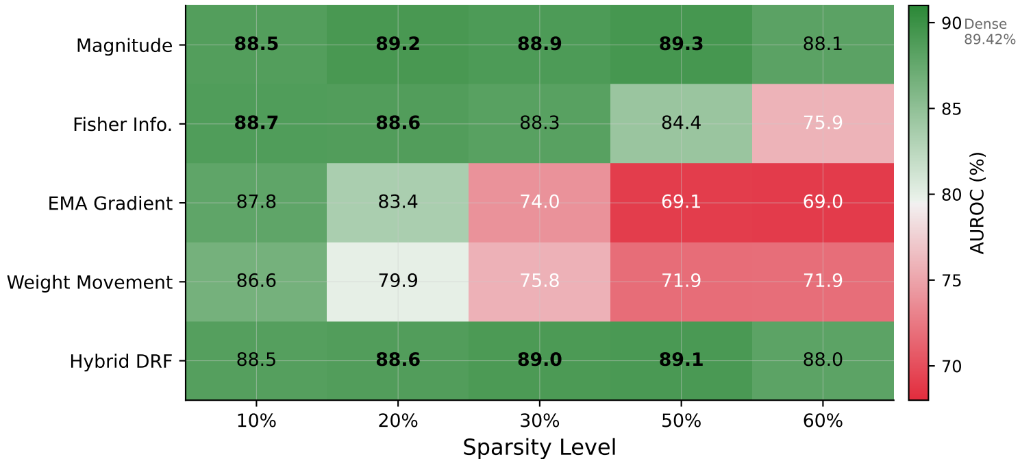
Validation AUROC (%) by Scorer and Sparsity Level
