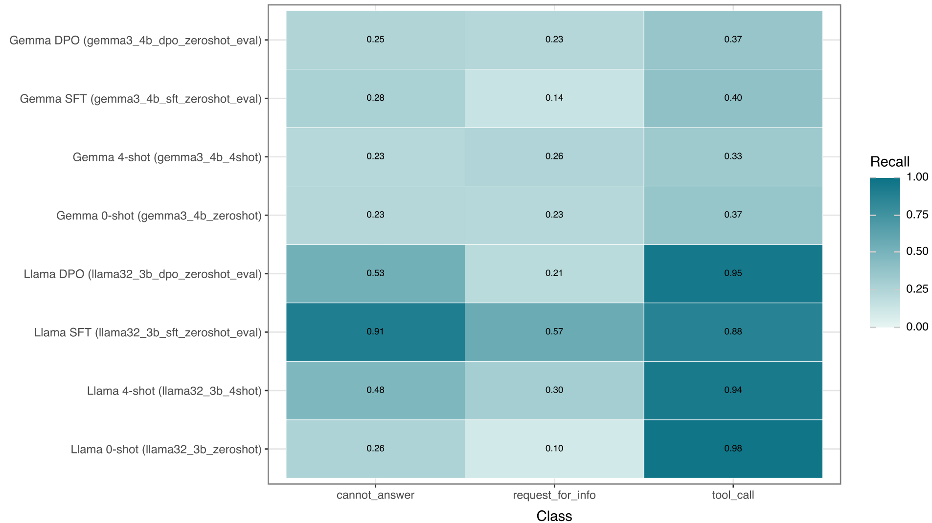
Per-Class Recall
