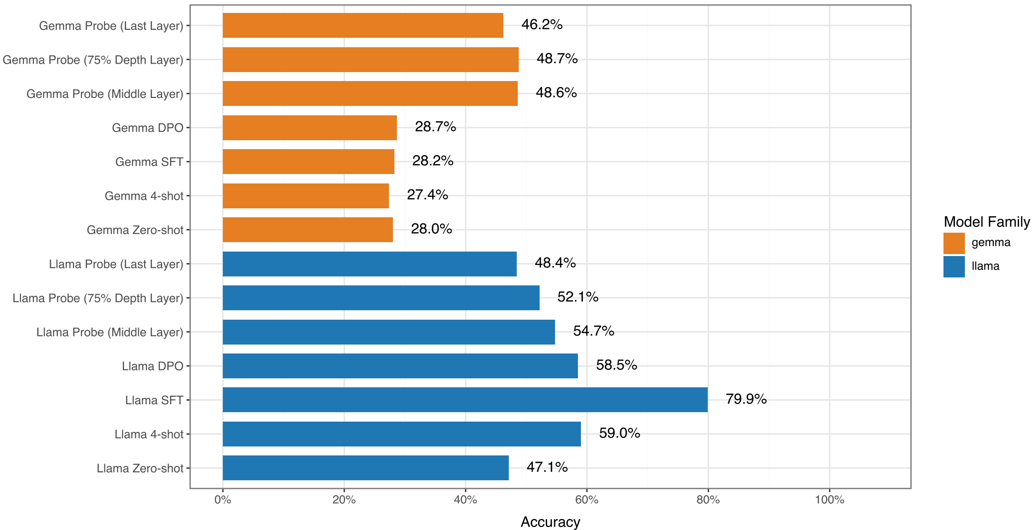
Normalized Accuracy by Run
