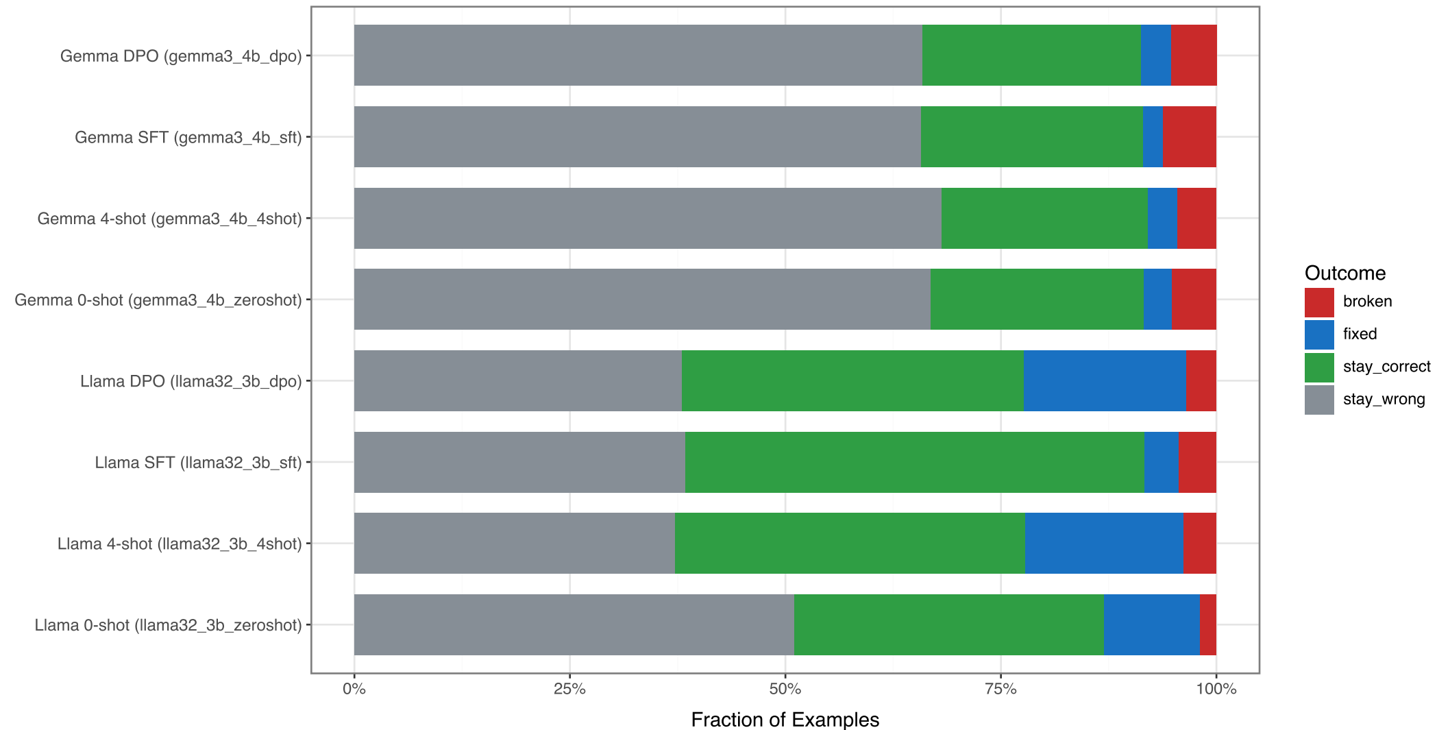
Normalization Outcome Breakdown
