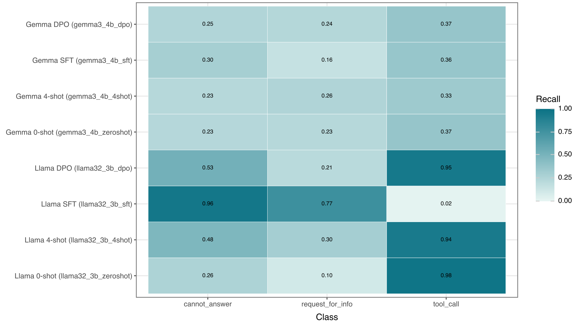
Normalized Recall by Class
