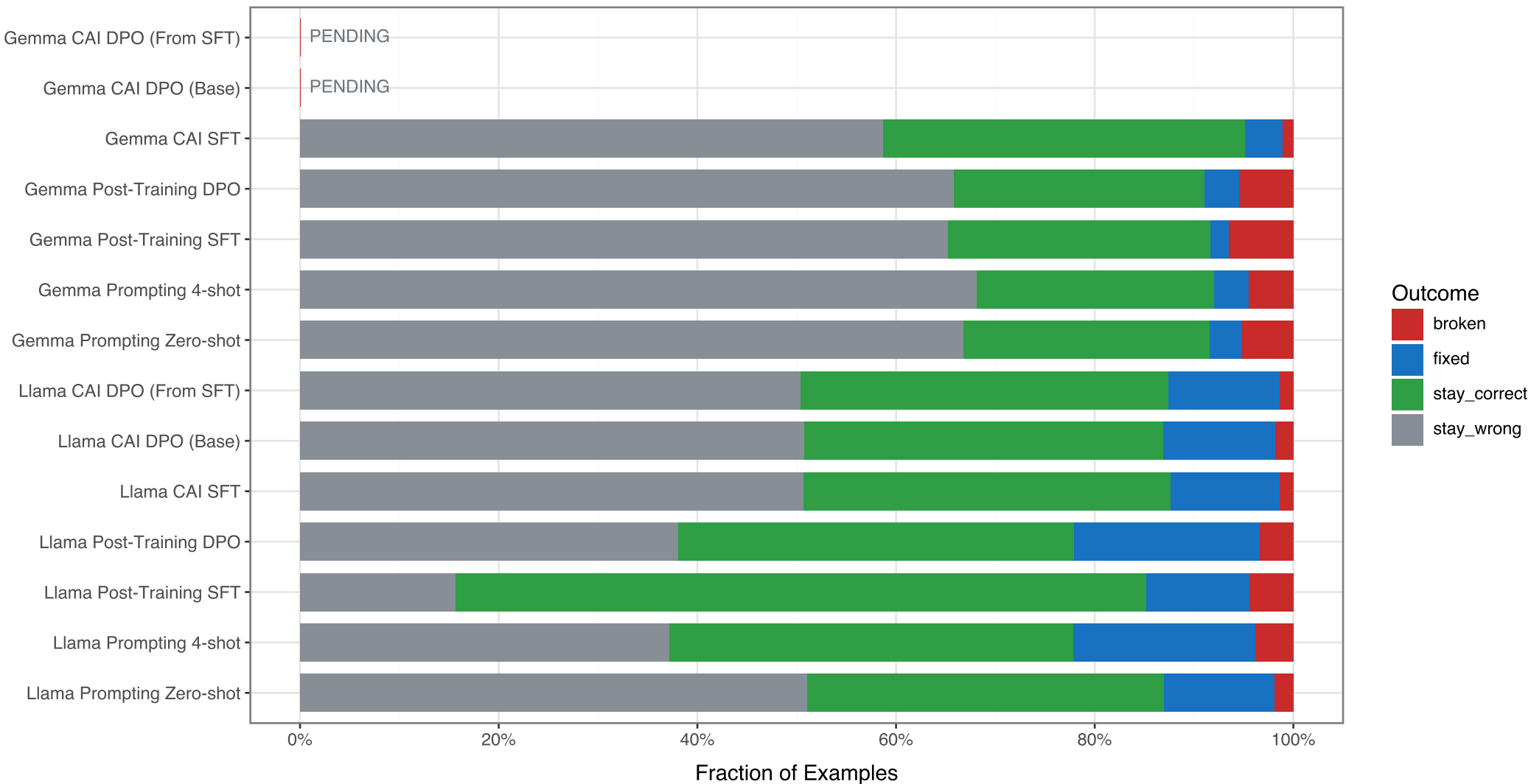
When2Call (hmm): Prompting + Post-Training + CAI - Normalization Outcome Breakdown (Without Probe)
