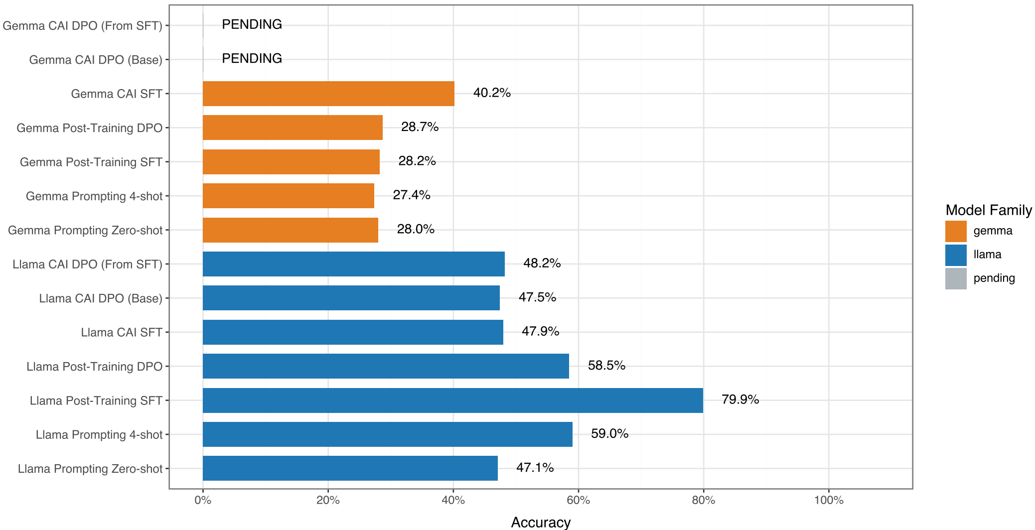
When2Call (hmm): Prompting + Post-Training + CAI - Normalized Accuracy by Run (Without Probe)
