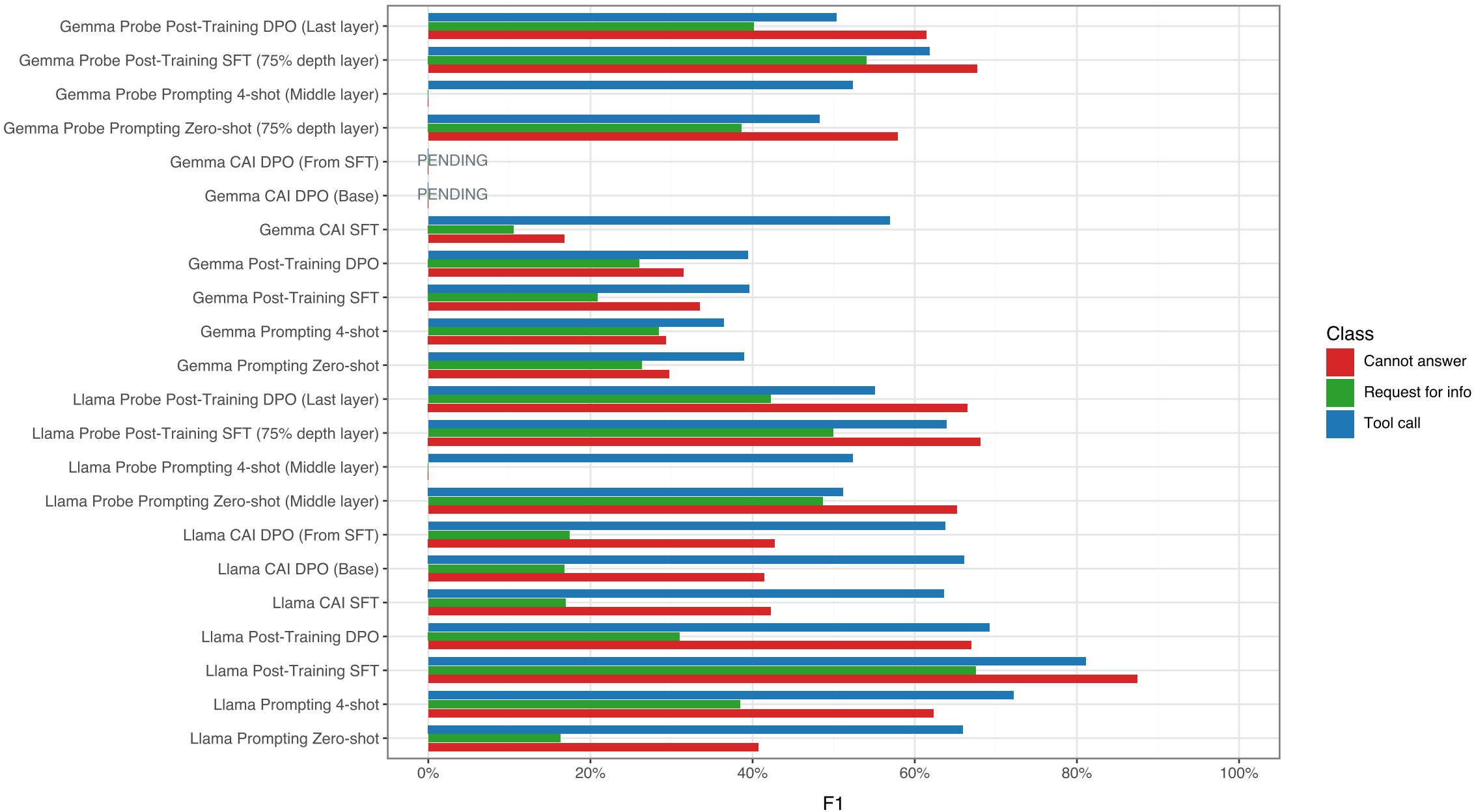
When2Call (hmm): Prompting + Post-Training + CAI + Probe - Per-Class F1 by Run (Normalized)
