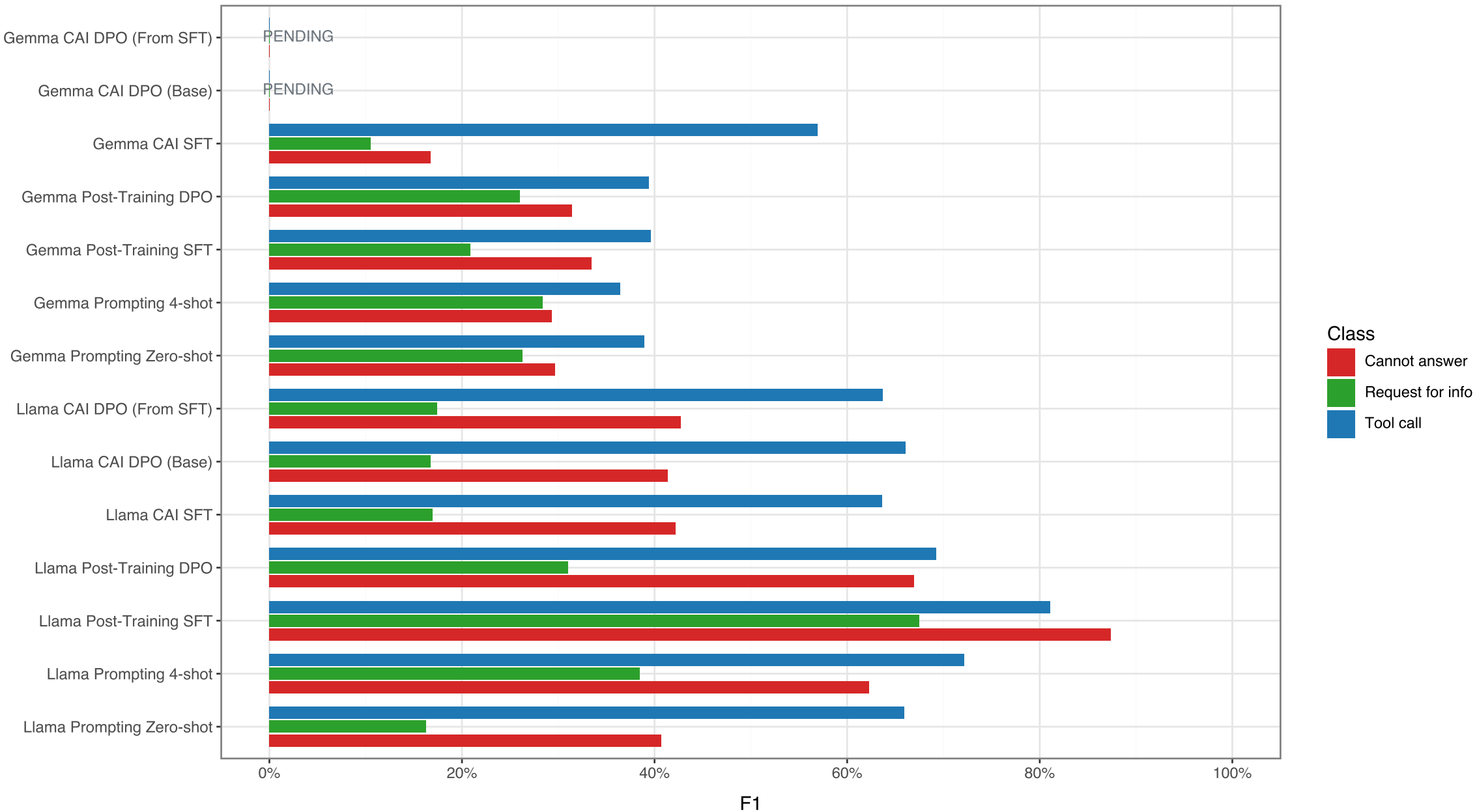
When2Call (hmm): Prompting + Post-Training + CAI - Per-Class F1 by Run (Normalized) (Without Probe)
