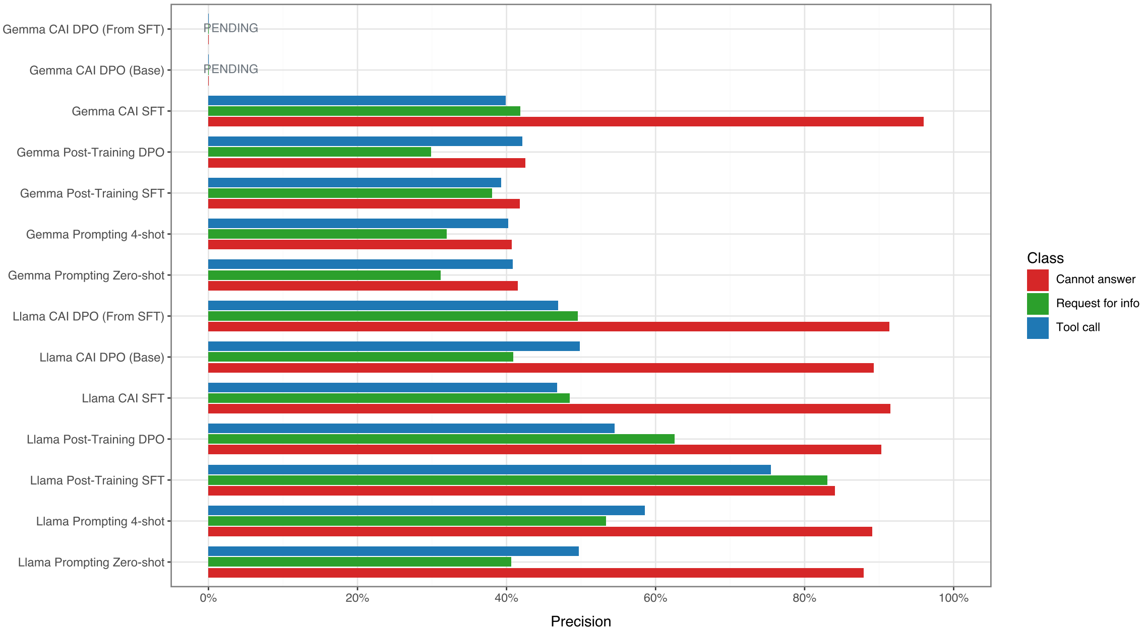
When2Call (hmm): Prompting + Post-Training + CAI - Per-Class Precision by Run (Normalized) (Without Probe)
